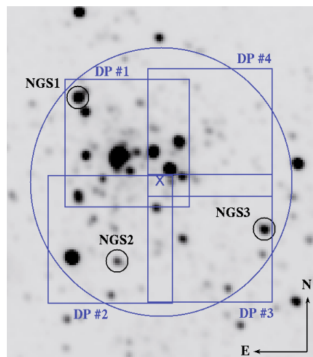
Fig. 1. 2MASS K band image of Tr 14. The cross and the large circle indicate the centre and the size of the 2' MAD field of view. The four 57'' \times 57'' boxes show the position of the CAMCAO camera in the adopted 4-point dither pattern, while the selected NGSs are identified by the smaller circles.
