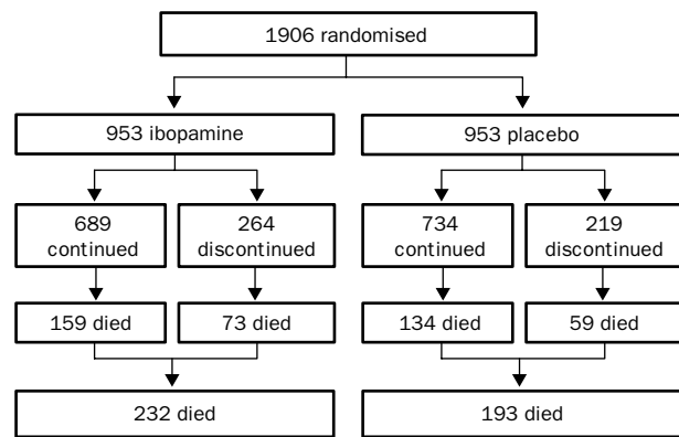
Figure 1: Trial profile
