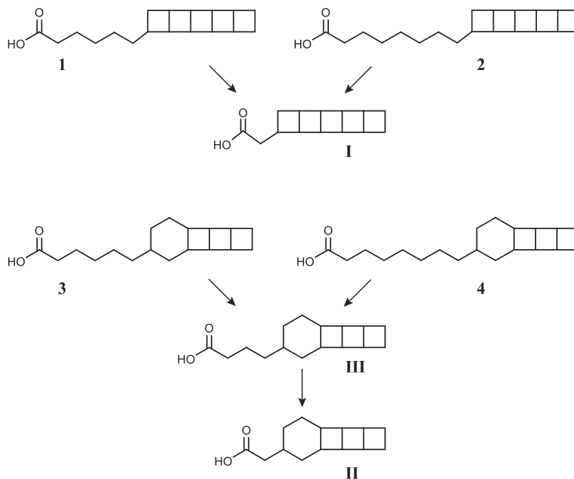
Fig. 1. Structures of ladderane lipids derived from anammox bacteria and their transformation products derived from microbial oxic degradation. (1) C 18 -[5]-ladderane FA, (2) C 20 -[5]-ladderane FA, (3) C 18 -[3]-ladderane FA, (4) C 20 -[3]-ladderane FA, (I) C 14 -[5]-ladderane FA, (II) C 14 -[3]-ladderane FA, (III) C 16 -[3]-ladderane FA. Key: FA = fatty acid.
