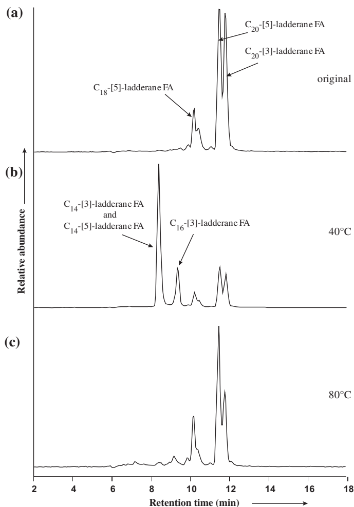
Fig. 5. HPLC base peak chromatograms of the fatty acid fraction (analyzed as their methyl ester derivatives) showing the distribution of ladderane fatty acids in anammox degradation experiments: original (a), heated for three days at 40 °C (b), and heated for 3 days at 80 °C (c).
