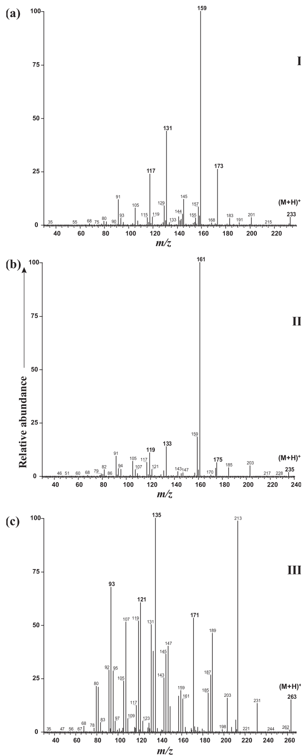
Fig. 6. APCI-MS/MS spectra of the protonated molecular ions of three different ladderane lipid transformation products: (a) component I ( m/z 233), (b) component II ( m/z 235), and (c) component III ( m/z 263). Structures of the original lipids and the alteration products are depicted in Fig. 1.
