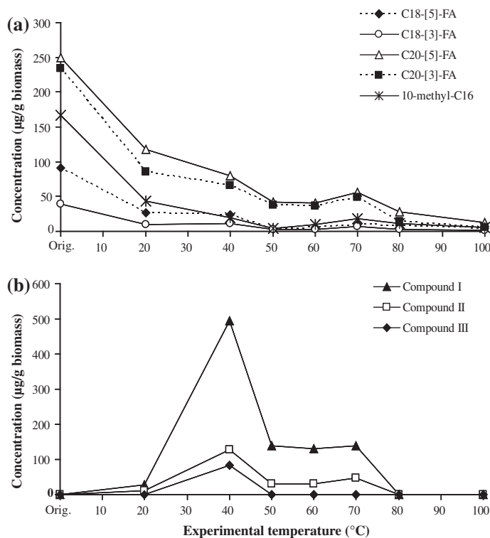
Fig. 3. Concentration of (a) known ladderane lipids and 10-methylhexadecanoic acid, and (b) short-chain ladderane transformation products as a function of temperature in the fatty acid fractions after base hydrolysis and analyzed by GC.
