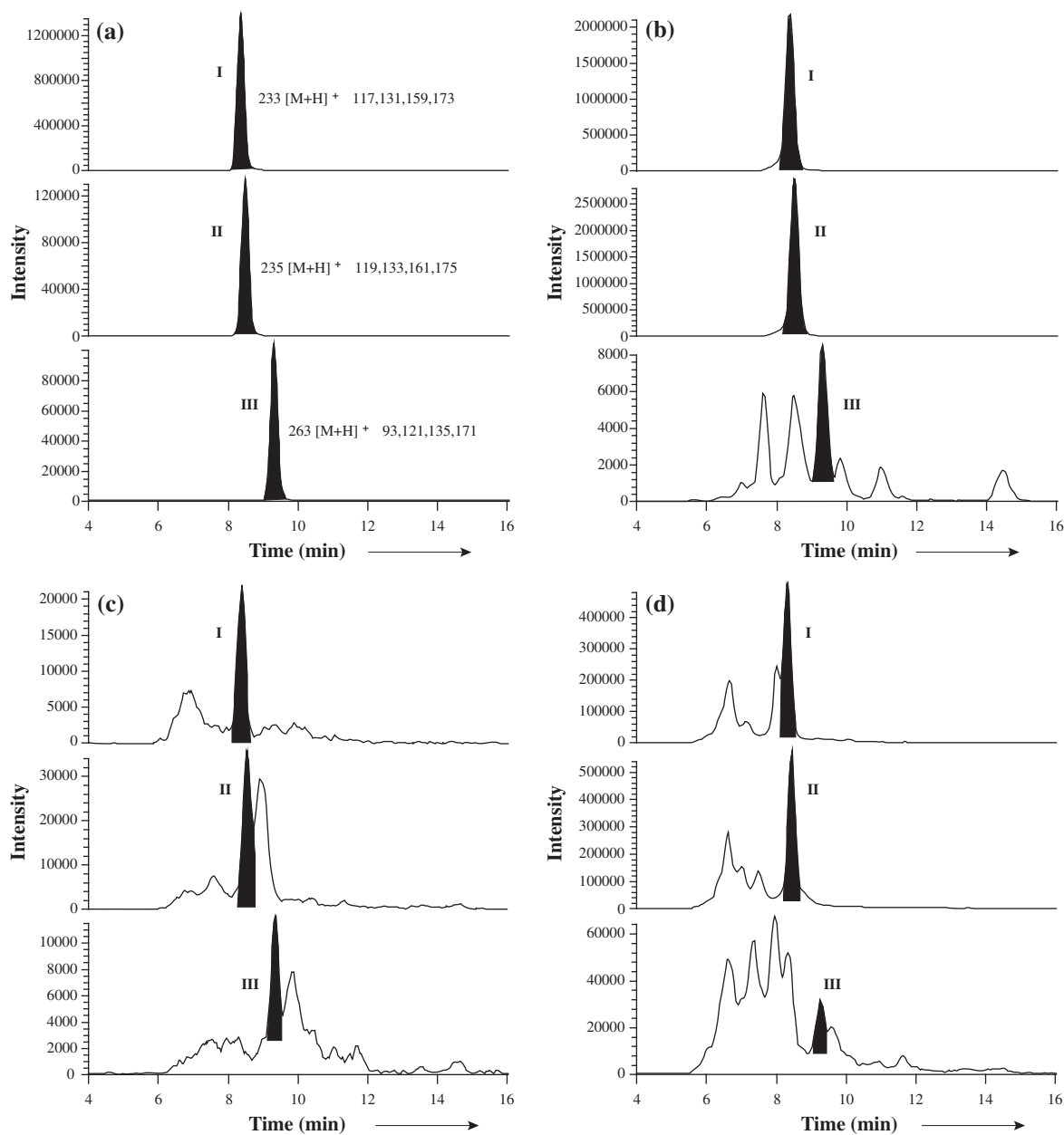
Fig. 7. SRM traces of short-chain ladderane fatty acids (analyzed as their methyl ester derivatives) in (a) anammox biomass heated at 40 °C for three days, and in sediments from (b) the Arabian Sea, (c) the Irish Sea, and (d) offshore northwest Africa.
