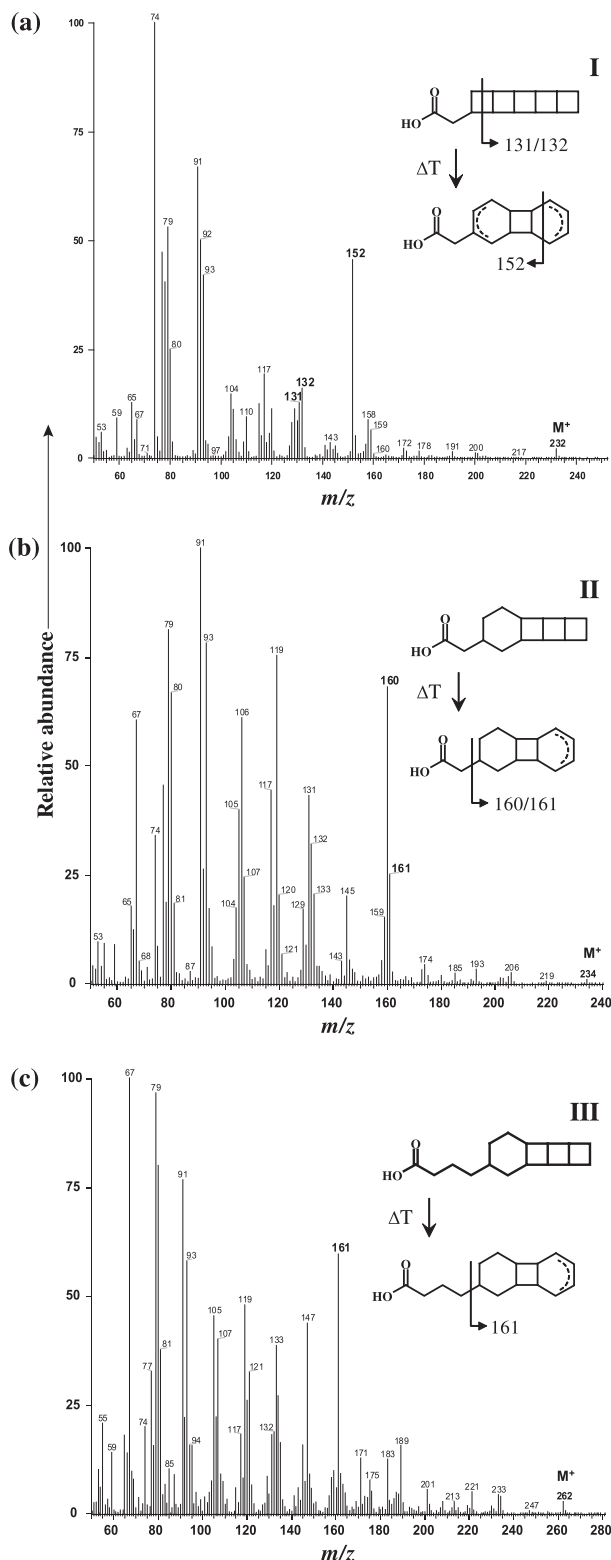
Fig. 4. GC/MS spectra of the short-chain ladderane fatty acids I , II , and III analyzed as their methyl ester derivatives. (a) C 14 -[5]-ladderane fatty acid, (b) C 14 -[3]-ladderane fatty acid, and (c) C 16 -[3]-ladderane fatty acid. It should be noted that the mass spectra reflect the thermal degradation products formed during GC analysis as discussed by Sinnighe Damsté et al. (2005).
