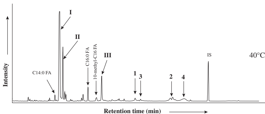
Fig. 2. Gas chromatogram of the fatty acid fraction of anammox biomass incubated for three days at 40^{\circ}\text{C} . Numbers correspond to structures shown in Fig. 1. IS denotes internal standard ( ante iso \text{C}_{22} alkane).
