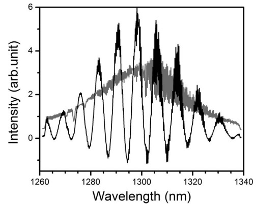
Fig. 2. Reference spectrum (gray curve) and interference spectrum (dark curve) after reference spectrum subtraction, both measured with the AWG spectrometer in the fiber-based SD-OCT.
