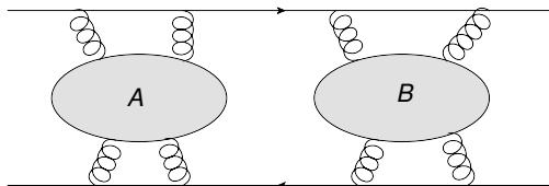
Figure 8. General form of a diagram which is two-eikonal-line reducible.
