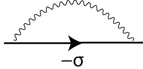
FIG. 5. The pseudofermion self-energy: solid line denotes G(i\epsilon_n) whereas wavy line stands for the interaction \alpha(i\omega_n) (see text).
