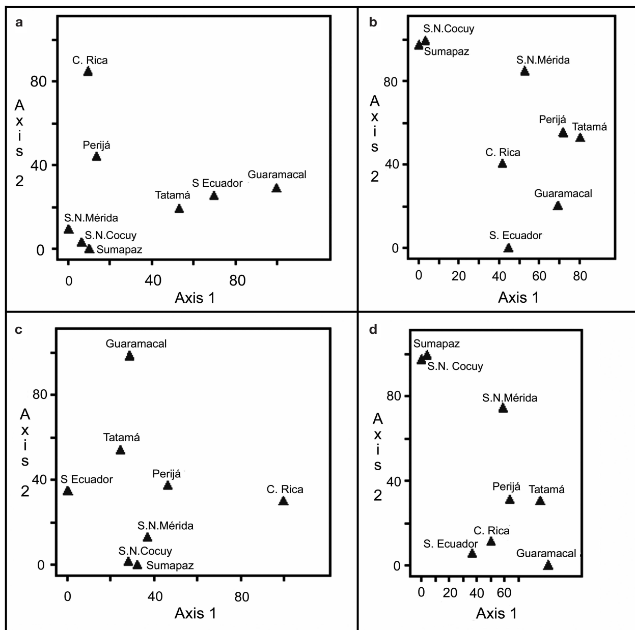
Fig. 4. DCA (a, c) and PCA (b, d) Ordination diagrams of 404 (a, b, including páramo & SARF genera from Guaramacal) and 347 (c, d, including only proper páramo genera from Guaramacal) genera for 8 páramo floras datasets. a , DCA Axis 1 Eig = 0.422; Axis 2 Eig = 0.321; b , PCA Axis 1 Eig = 473.827; Axis 2 Eig = 121.424; c , DCA Axis 1 Eig = 0.223; Axis 2 Eig = 0.189; d , PCA Axis 1 Eig = 803.377; Axis 2 Eig = 87.539.
