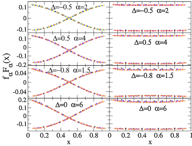
FIG. 5 (color online). Universal scaling function f_\alpha F_\alpha(x) (where x = \ell/L ) for the XXZ chain for several values of \alpha and \Delta . Left: Several \alpha and \Delta for odd L . Right: even L . In the latter case, F_\alpha(x) is practically independent on x .
