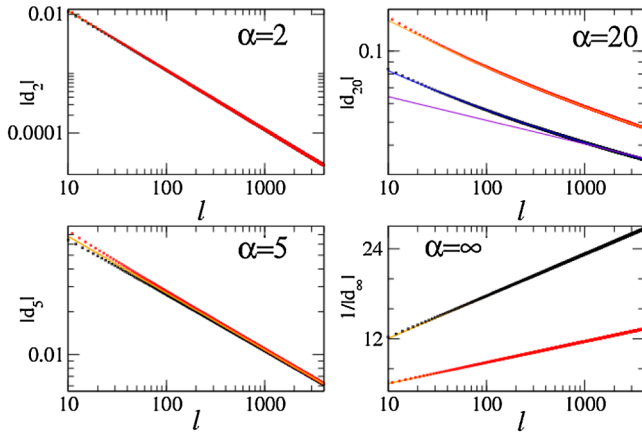
FIG. 2 (color online). Corrections to scaling d_\alpha(\ell) = S_\alpha(\ell) - S_\alpha^{\text{CFT}}(\ell) for the XX model and four different values of \alpha . Red circles and black squares correspond to even and odd \ell , respectively.
