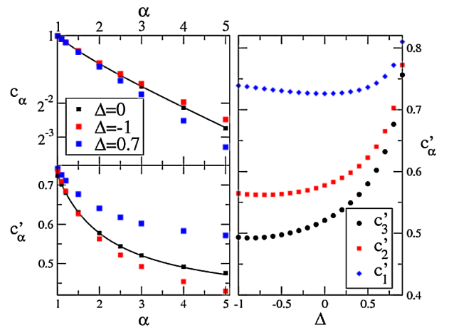
FIG. 4 (color online). Left: The additive constant in the Rényi entropies c'_\alpha (bottom) and the multiplicative constant c_\alpha for the moments \text{Tr} \rho_A^\alpha (top in log scale) as function of \alpha at fixed \Delta . The drawn lines are the exact values for \Delta = 0 . Right: c'_\alpha as function of \Delta at fixed \alpha .
