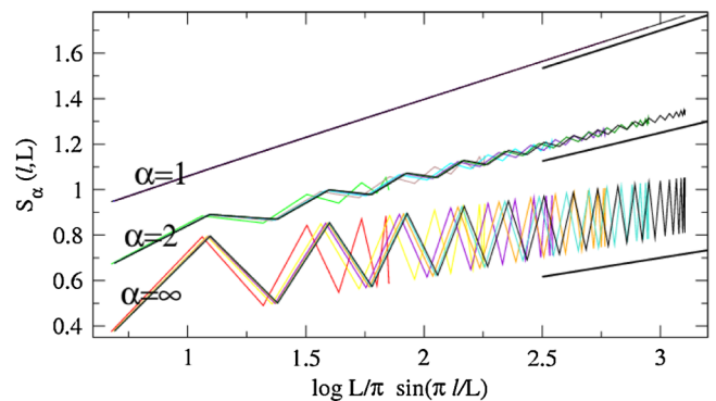
FIG. 1 (color online). Parity effects in Rényi entropies in the XXZ model at \Delta = -1/2 . S_\alpha(\ell, L) for several L and \alpha = 1, 2, \infty . The straight lines indicate the asymptotic slopes (1 + \alpha^{-1})/6 .
