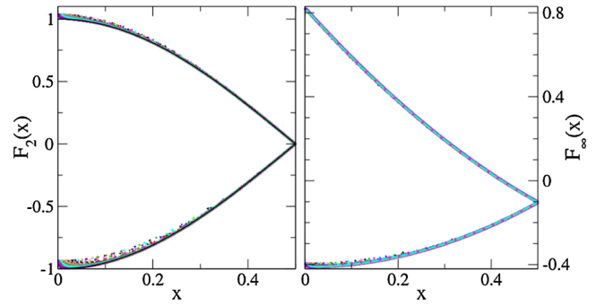
FIG. 3 (color online). Corrections to scaling in the finite length XX model for odd L . F_2(x) and F_\infty(x) ( x = \ell/L ) obtained from 69 different systems with lengths in the range 17 \leq L \leq 4623 exhibit perfect data collapse.
