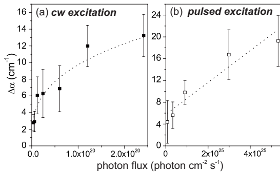
FIG. 5. Laser-induced absorption coefficient changes \Delta\alpha as function of the excitation photon flux \Phi for both (a) cw and (b) pulsed excitation ( t_p=5 \text{ ns} ) at 532 \text{ nm} . The dashed lines represent fits by Eqs. (7) and (9), respectively.
