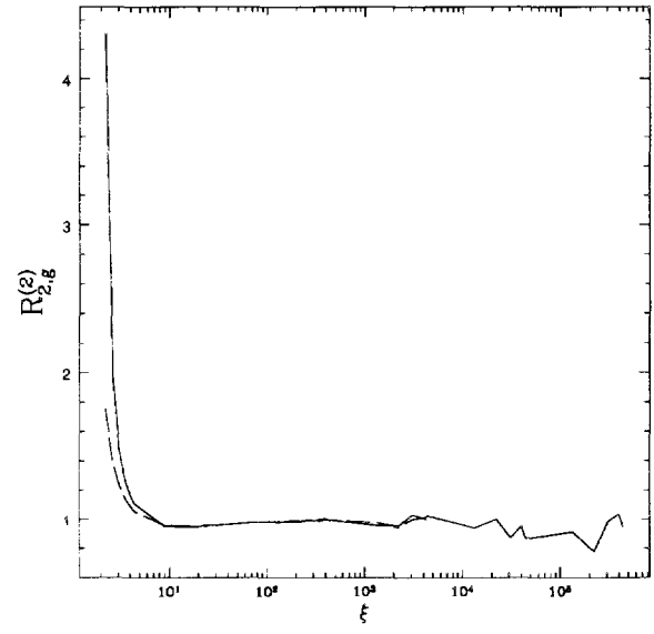
Figure 2. R_{2,g}^{(2)} plotted as a function of \xi for fixed z = 10^{-2} (solid line) and for z = 10^{-4} (dashed line).
