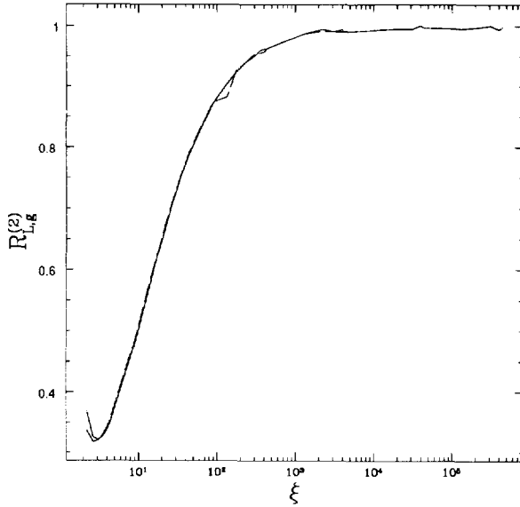
Figure 1. R_{L,g}^{(2)} plotted as a function of \xi for fixed z = 10^{-2} (solid line) and for z = 10^{-4} (dashed line).
