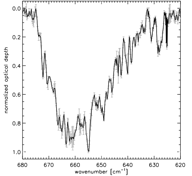
Fig. 9. 15.25 \mu\text{m} \text{CO}_2 bending mode observed by ISO in IRAS 06084-0611. The uncertainties are indicated in grey.
