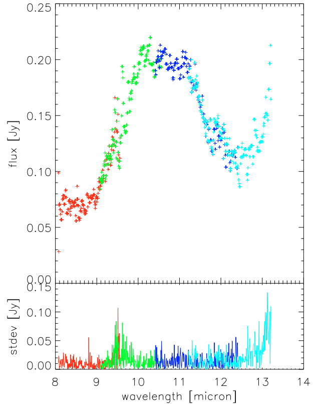
Fig. 7. VISIR spectrum of HD 176386 Position 1, median smoothed over 5 elements.
