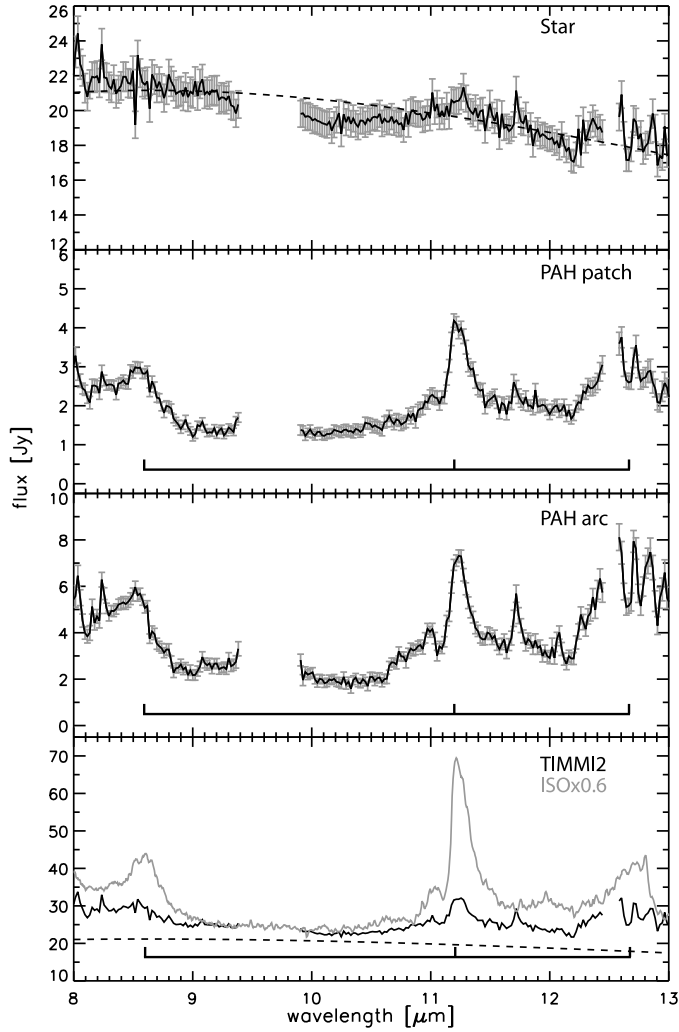
Fig. 4. The TIMMI2 spectra of the three components of CD-42 11721 (see Figs. 1 and 2, and Sect. 3.2) are shown in the top three panels. The fourth panel shows a comparison of the TIMMI2 spectrum of the four emission peaks combined with the ISO-SWS spectrum. The dashed lines show the fit made to the star ( \log(F) = a + b \times \lambda with a = -15.201 \pm 0.008 , b = -0.1006 \pm 0.0008 and F in \text{W cm}^{-2} ). Indicated are the 8.6, 11.2 and 12.7 \mu\text{m} PAH bands.
