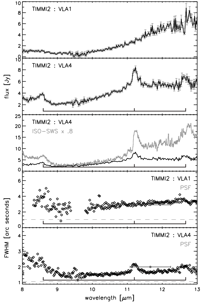
Fig. 3. The top two panels show the TIMMI2 spectra of IRAS 06084-0611 VLA1 and VLA4. A comparison between the ISO-SWS spectrum and the TIMMI2 spectra of IRAS 06084-0611 VLA4 (see Fig. 1 for the apertures) is plotted in the middle panel . The lower two panels show the FWHM of both sources as a function of wavelength (black diamonds), the FWHM of the sources in the 11.9 \mu\text{m} image in the slit direction (grey dot) and the FWHM of the calibration star (dashed grey line). Indicated are the 8.6, 11.2 and 12.7 \mu\text{m} PAH bands.
