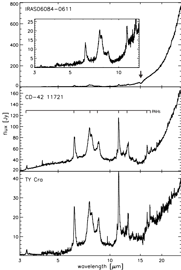
Fig. 8. ISO-SWS spectra of IRAS 06084-0611, CD-42 11721 and TY CrA. Indicated are the 3.3, 6.2, “7.7”, 8.6, 11.2, 12.7, 16.4 and 17.4 \mu\text{m} PAH bands. The arrow indicates the 15.25 \mu\text{m} \text{CO}_2 bending mode, see Fig. 9 for a detailed profile.
