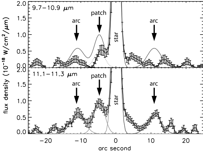
Fig. 2. Two spatial cross-cuts of the TIMMI2 spectra of CD-42 11721. The top panel plots the continuum between 9.7 and 10.9 \mu\text{m} , and the bottom panel plots the 11.2 \mu\text{m} PAH band between 11.1 and 11.3 \mu\text{m} . Several wavelength rows have been collapsed to reduce the noise. The grey line (in both panels) represents a fit to the PAH cross-cut with 4 Gaussians. The dotted line in the top panel is a scaled version of the Gaussian peaking at \sim -4.7'' . The PAH emission from the arc peaks around \pm 11'' . Finally, the data reveals a separate, independent patch of emission which peaks around \sim -5'' , near the central star.
