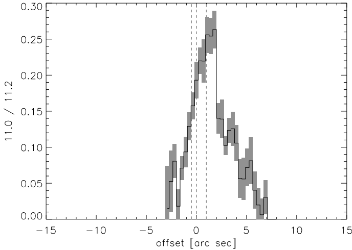
Fig. 13. 11.0/11.2 \mu\text{m} PAH band strength ratios of TY CrA as a function of position. The dashed lines at -0.5 , 0.0 and 1.0'' trace the 11.2 \mu\text{m} , continuum and second 8.6 \mu\text{m} peaks from Fig. 12, respectively.
