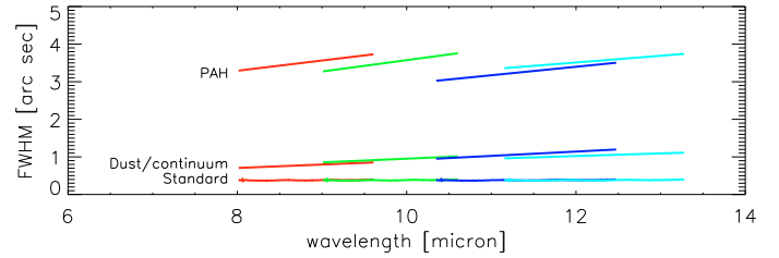
Fig. 6. FWHM as a function of wavelength of the amorphous silicate and PAH components in TY CrA. Also shown is the FWHM of the calibrator as a function of wavelength.
