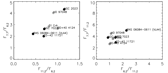
Fig. 15. Left: F_{11.2/6.2} versus F_{7.7/6.2} PAH band strength ratio. Right: F_{6.2/11.2} versus F_{7.7/11.2} PAH band strength ratio. The reflection nebulae are shown in black and the Herbig Ae/Be stars in grey.
