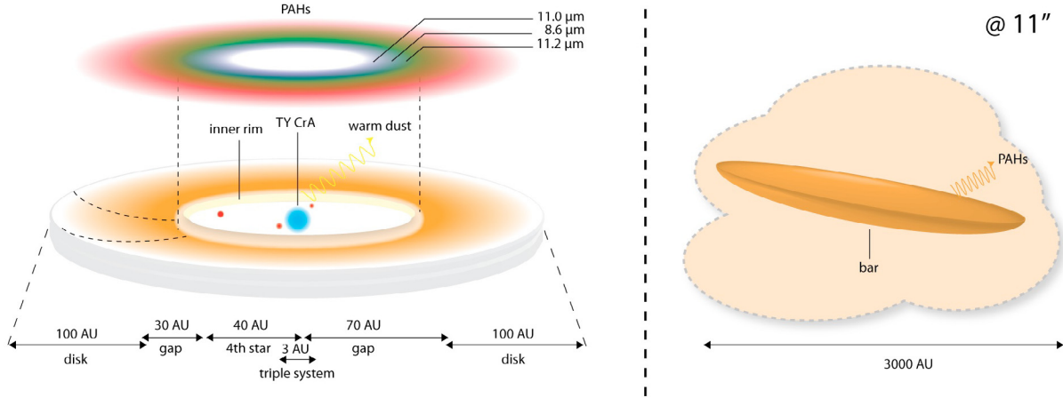
Fig. 14. Cartoon of the proposed morphology for TY CrA depicting the different emission zones.
