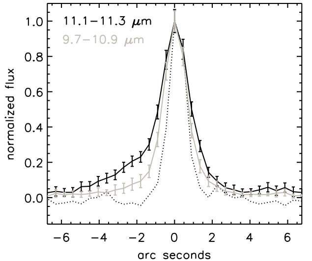
Fig. 10. Spatial distribution of IRAS 06084-0611 VLA4 (solid line) and the calibration star (dotted line) from TIMMI2 at 11.22 \mu\text{m} (black). This is compared to the spatial distribution at 10.5 \mu\text{m} (grey). For the continuum, the pixel rows from 9.7 to 10.9 \mu\text{m} were summed; for the PAH band, pixel rows from 11.1 to 11.3 \mu\text{m} were summed.
