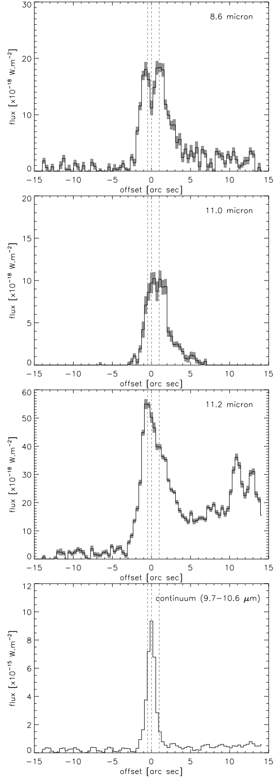
Fig. 12. Integrated band strength as a function of position for the 8.6 , 11.0 and 11.2\ \mu\text{m} PAH features and the continuum in TY CrA. The dashed lines at -0.5 , 0.0 and 1.0'' trace the 11.2\ \mu\text{m} , continuum and second 8.6\ \mu\text{m} peaks, respectively, across all panels.
