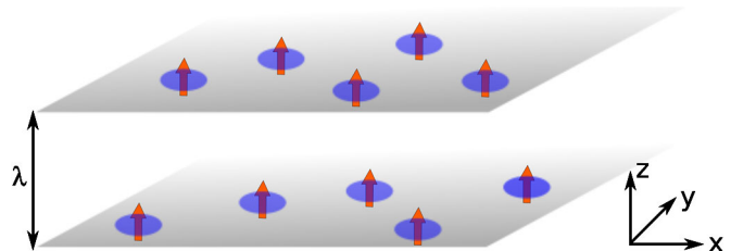
FIG. 1 (color online). Bilayer dipolar system under consideration.
