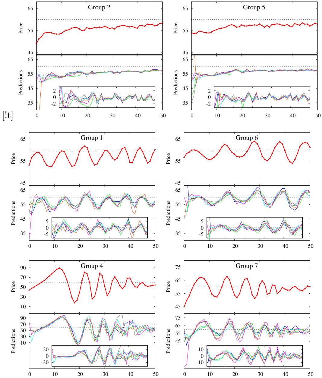
Figure 6: Asset Pricing LtFEs in six different groups. The top part of each panel shows realized market prices, the middle part shows six individual predictions and the bottom part of each panel shows the individual forecast errors.
