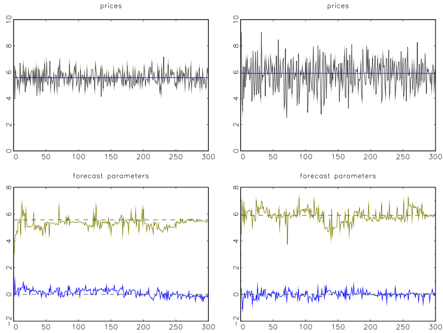
Figure 4: Simulated prices (top panels) and average parameters \alpha and \beta of the AR1 forecasting rules (3.7) under GA-learning (bottom panels). In the stable treatment (left panels) price volatility is low and parameters remain close to the RE-benchmark ( \alpha = 5.57 and \beta = 0 ), while in the unstable treatment (right panels) price volatility is high and GA-learning does not converge to the RE benchmark ( \alpha = 5.91 and \beta = 0 ).
