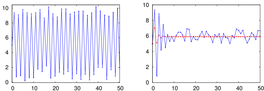
Figure 2: Cobweb dynamics in the strongly unstable treatment ( \lambda = 2 ) in two benchmark simulations. Left Panel: convergence to a (noisy) 2-cycle under naive expectations. Right Panel: convergence to (noisy) RE equilibrium price under learning by average.
