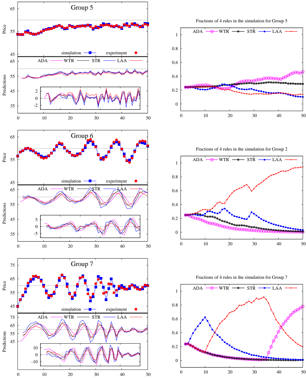
Figure 8: Left Panels: realized prices for laboratory experiments in different groups (red) with corresponding one-step ahead predictions of the heuristics switching model (blue). Lower parts of left panels show predictions and forecasting errors (inner frames) of the four heuristics. Right Panels: Evolution of the fractions of the 4 heuristic during the one-step ahead predictions of the model: adaptive expectations (ADA, purple), weak trend followers (WTR, black), strong trend followers (STR, blue) and anchoring adjustment heuristic (LAA, red).
