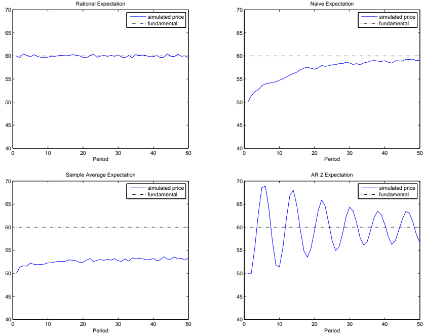
Figure 5: Homogeneous expectations benchmarks: Top Panels RE (left) and naive expectations (right); Bottom Panels: average expectations (left) and AR2 trend following rule p_{t+1}^e = (60 + p_{t-1})/2 + (p_{t-1} - p_{t-2}) .
