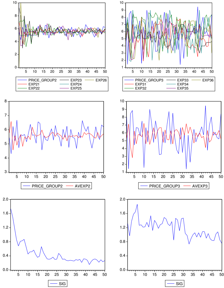
Figure 3: Cobweb Learning to Forecast Experiments, typical session in stable treatment ( \lambda = 0.22 , left panels) and strongly unstable treatment ( \lambda = 2 , right panels). Top Panels: in stable treatment individual predictions coordinate on RE, while in unstable treatment heterogeneity in individual forecasting persists. Middle Panels illustrate average predictions and realized prices. Bottom Panels: degree of heterogeneity measured by standard deviations of individual forecasts (6 individuals) averaged over the six groups in each treatment.
