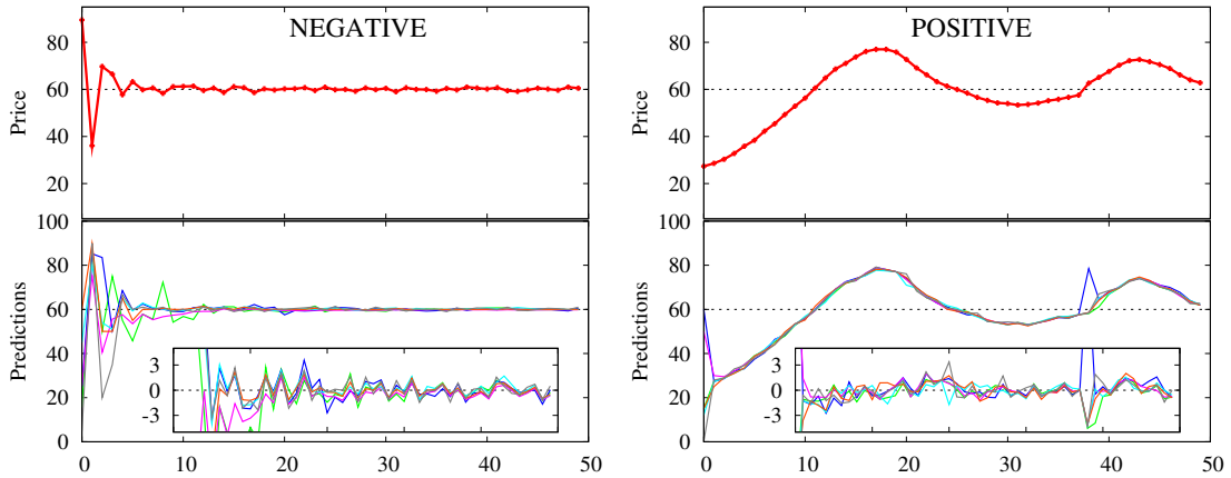
Figure 9: Negative (left panel) vs. positive (right panel) feedback Learning-to-Forecast-Experiments with small IID shocks; prices (top panels), individual predictions (bottom panels) and forecast errors (small panels).
