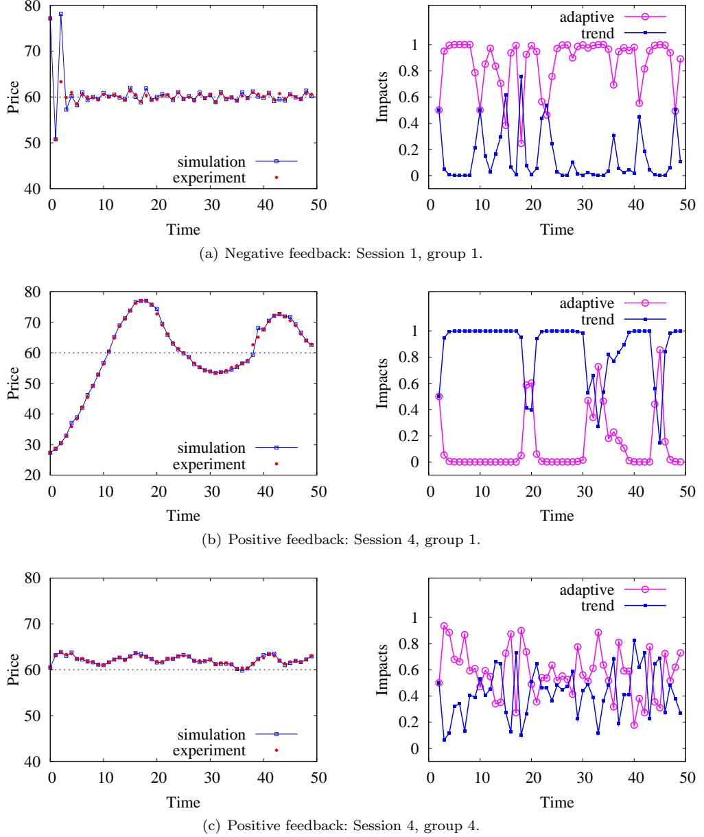
Fig. 5 Dynamics of the HHST experiment as compared with the one-period ahead predictions by the heuristic switching model, augmented by experimental noise. The parameters are w = 0.75 , \gamma = 1 , \beta = 1.5 , \delta = 0.1 and \eta = 0.1 . Left : Price dynamics in the experiment (points) and forecasts generated by the model (line). Right : Evolution of impacts of two heuristics.
