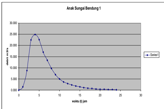
Figure 3. Unit Hydrograph Synthetic of Bendung watershed [12]
