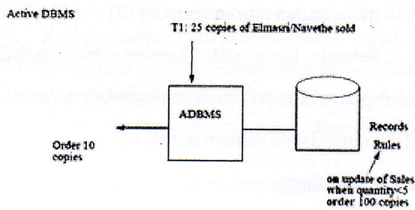
Gambar 2. Model Active Database
