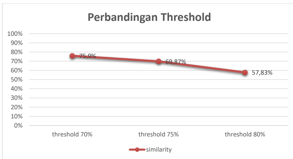
Gambar 3.1 Diagram similarity
