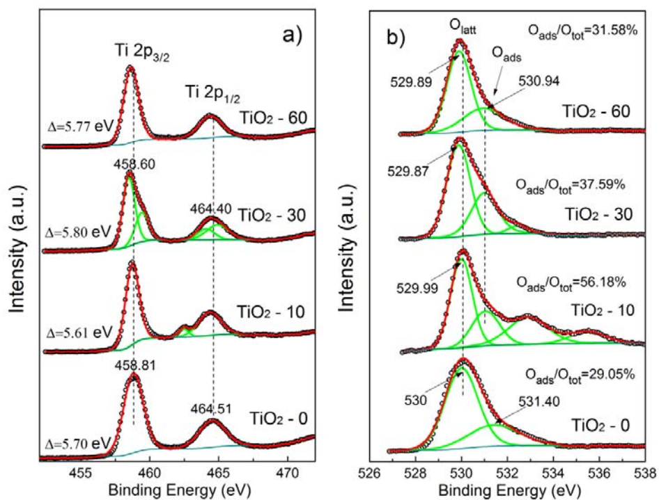
Figure 4. a) Ti 2p and b) O 1s high resolution XPS spectra of non-activated and mechanically activated TiO 2 . Mark \Delta stands for BE(2p_{1/2})-BE(2p_{3/2}) , while marks O_{latt} , O_{ads} and O_{tot} refer to the lattice oxygen, surface oxygen species and total oxygen in the material, respectively
