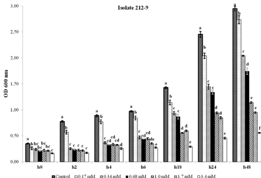
Figure 4. The growth kinetics of the Bacillus thuringiensis isolate 212-9 in liquid medium supplemented with different initial Cr(VI) concentrations. Values followed by the same letter within columns, within each time point of sampling, are not significantly different ( P < 0.05 ), according to Tukey's HSD test.
