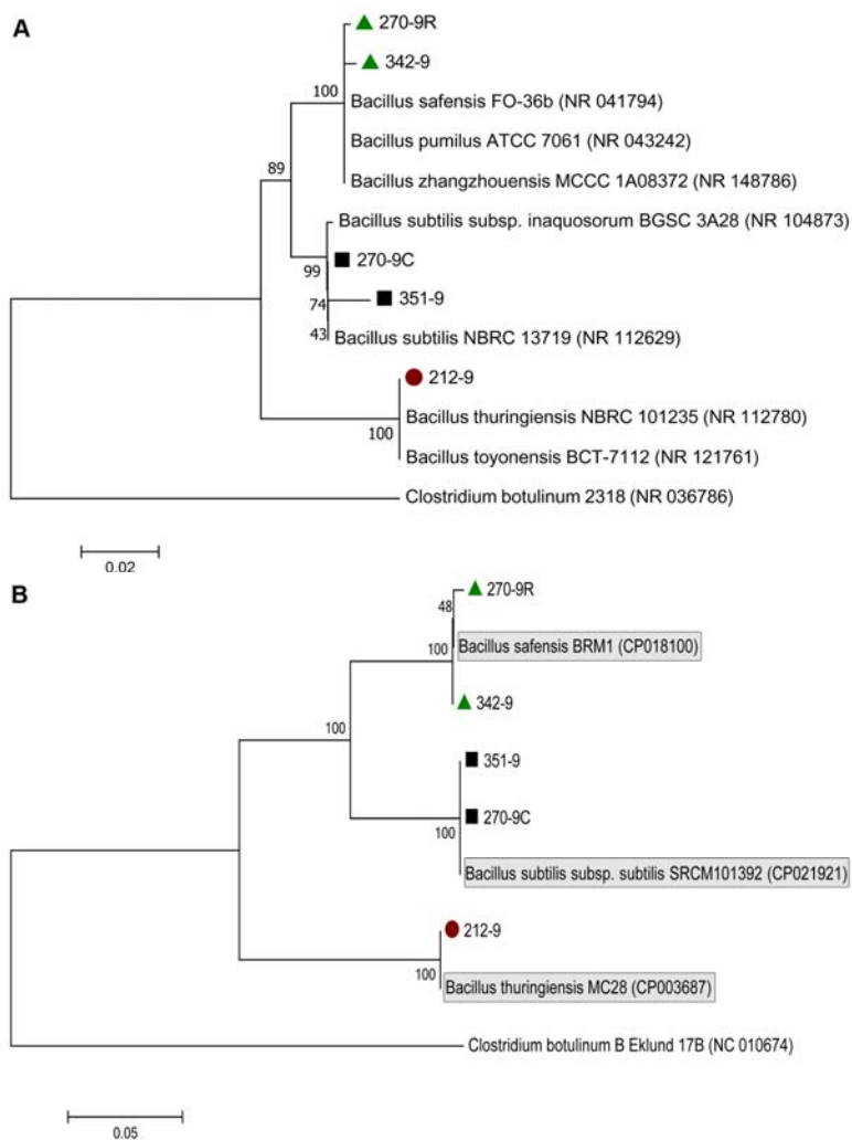
Figure 1. Neighbor-joining phylogenetic tree based on 16S rDNA (A) and tuf gene sequences (B) (1500 and 791 bp, respectively) showing the relationship of the tested isolates (212-9, 342-9, 270-9R, 351-9 and 270-9C) and related reference strains of the genus Bacillus . Clostridium botulinum (NR_036786 and NC_010674) was used as an out-group. Bootstrap values (expressed as a percentage of 1000 repetitions) are displayed at points of branching. The horizontal bar indicates a genetic distance of 0.02 for 16S rDNA and 0.05 for tuf gene.
