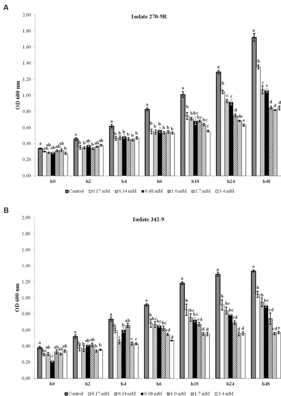
Figure 2. The growth kinetics of the Bacillus safensis isolates 270-9R (A) and 342-9 (B) in liquid medium supplemented with different initial Cr(VI) concentrations. Values followed by the same letter within columns, within each time point of sampling, are not significantly different ( P < 0.05 ), according to Tukey's HSD test.
