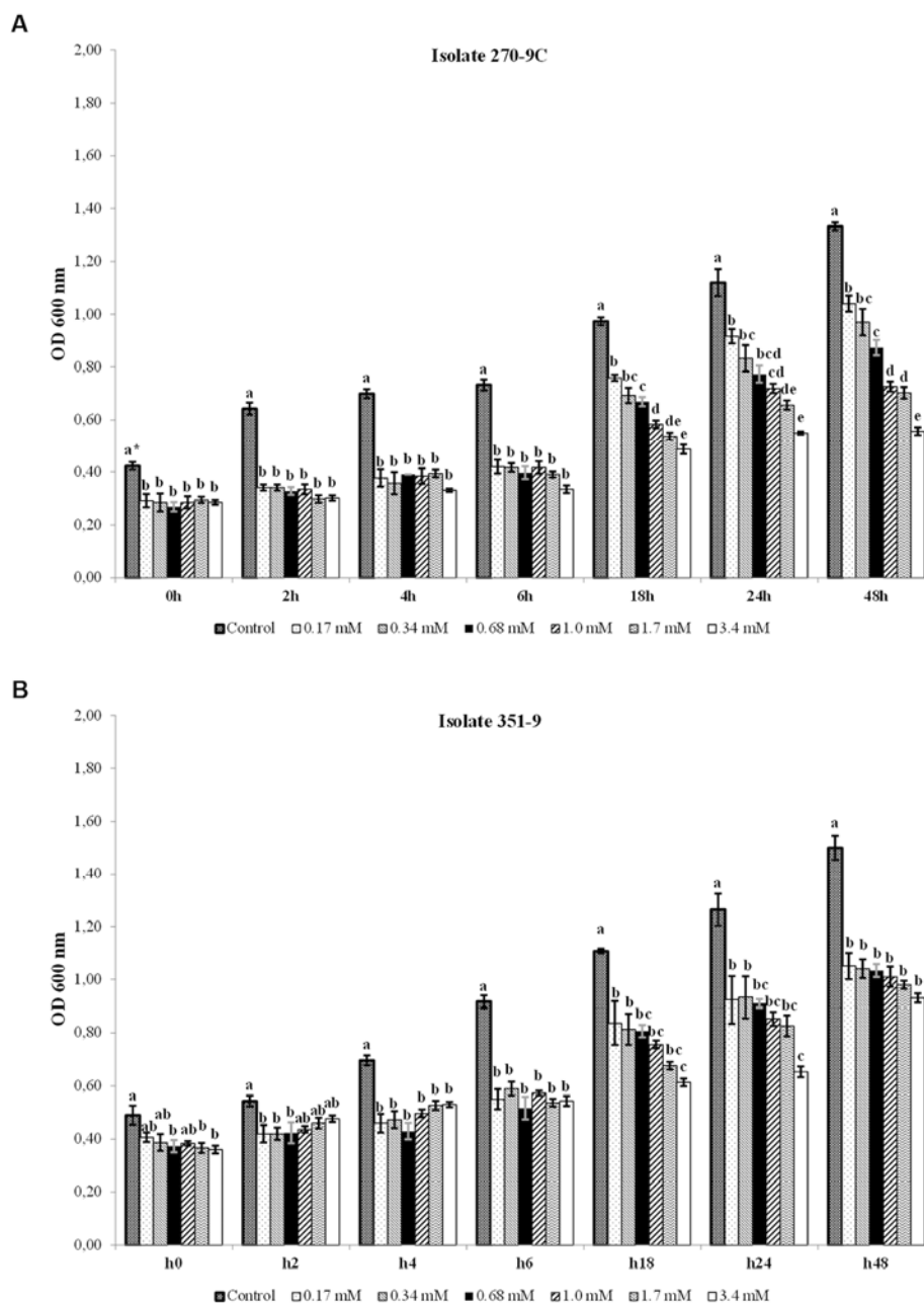
Figure 3. The growth kinetics of the Bacillus subtilis subsp. subtilis isolates 270-9C (A) and 351-9 (B) in liquid medium supplemented with different initial Cr(VI) concentrations. Values followed by the same letter within columns, within each time point of sampling, are not significantly different ( P < 0.05 ), according to Tukey's HSD test.
