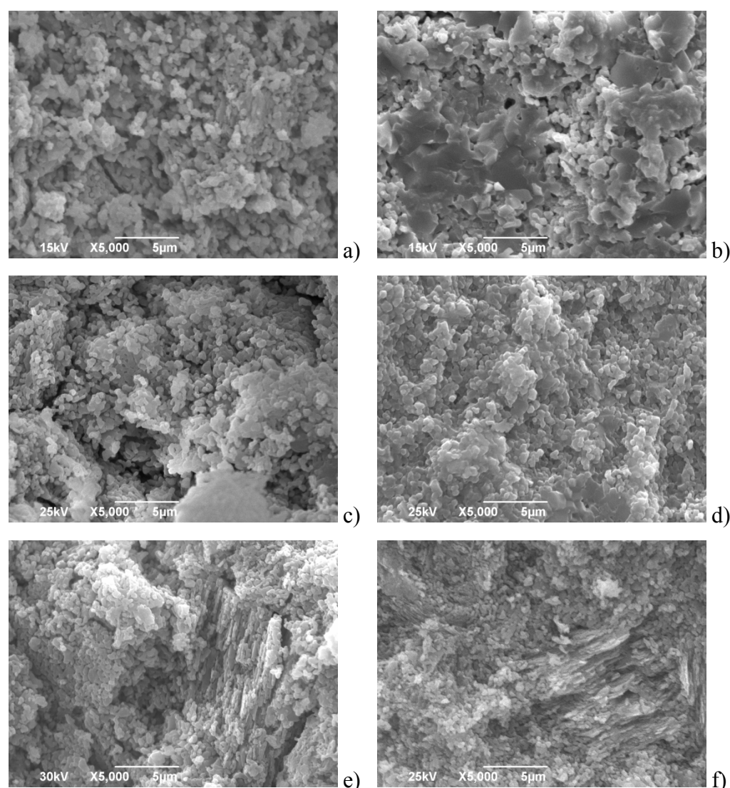
Fig. 3. SEM micrographs of sintered samples: a) AM-1-1400, b) AM-60-1400, c) AC-1-1400, d) AC-60-1400, e) AN-1-1400 and f) AN-60-1400.
