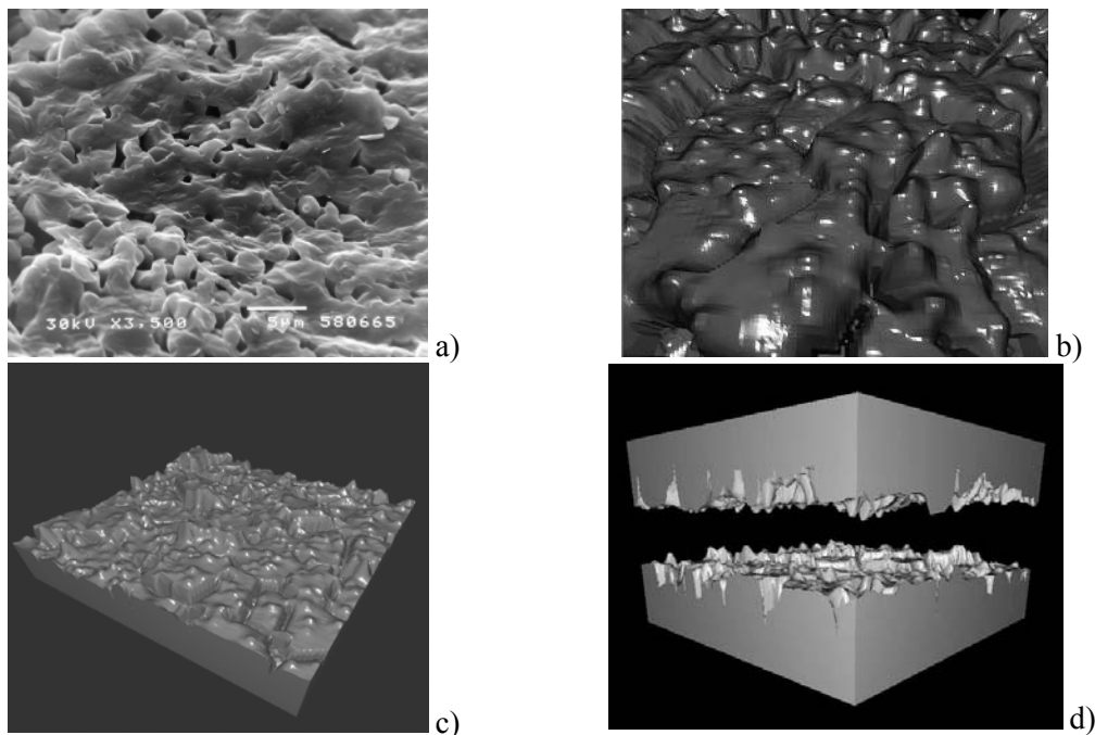
Fig. 7. a) SEM image of Yb doped BaTiO 3 ceramic, b) micro surface overview profile and c), d) 3D microsurface overview.
