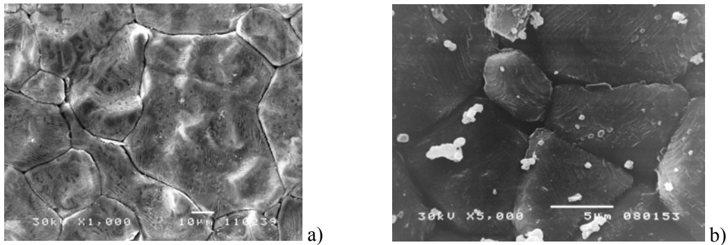
Fig. 4. SEM images of Yb doped BaTiO 3 sintered at 1380°C, doped with 0.1wt% and b) 1.0wt% of Yb.
