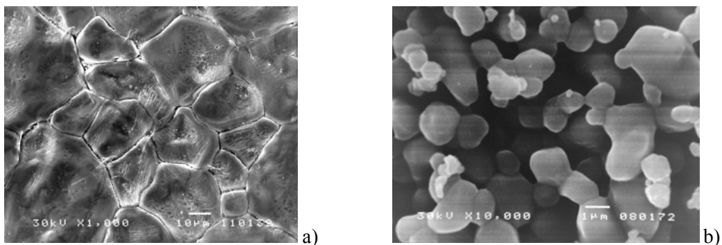
Fig. 3. SEM images of Yb doped BaTiO 3 sintered at 1350°C, doped with 0.1wt% and b) 1.0wt% of Yb.
