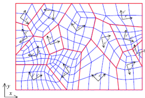
Fig. 1. Voronoi tessellation of 14-grain aggregate with grain boundaries, orientations of crystal lattices, finite element mesh and boundary conditions.
