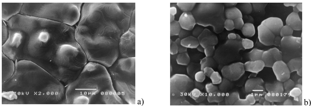
Fig. 2. SEM images of Yb doped BaTiO 3 sintered at 1320°C, doped with 0.1wt% and b) 1.0wt% of Yb.
