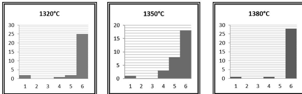
Fig. 8. Histograms corresponding to relevant statistical parameters for 0.1 Yb/BaTiO 3 samples, sintered at: a) 1320°C, b) 1350°C and c) 1380°C.
