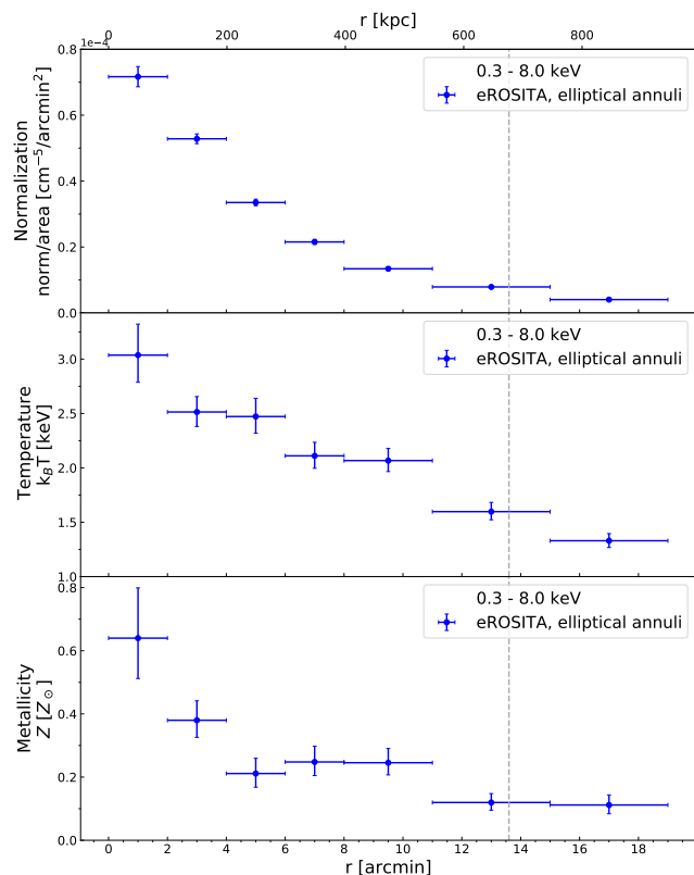
Fig. 6. Normalization (top), temperature (middle), and metallicity (bottom) profiles of A3408 using elliptical annuli, where r represents the semi-major axis. The grey dashed lines indicate the r_{500} of the cluster.
