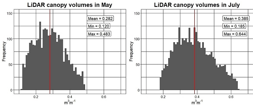
Figure 7. Absolut frequencies of LiDAR measurements with a interval of 0.01 \text{ (m}^3 \text{ m}^{-1}) . Such measurements were part of the software output (CSV file) where tractor, coupled with LiDAR, travelled completely four vine-rows. The red line corresponds to the mean value.
