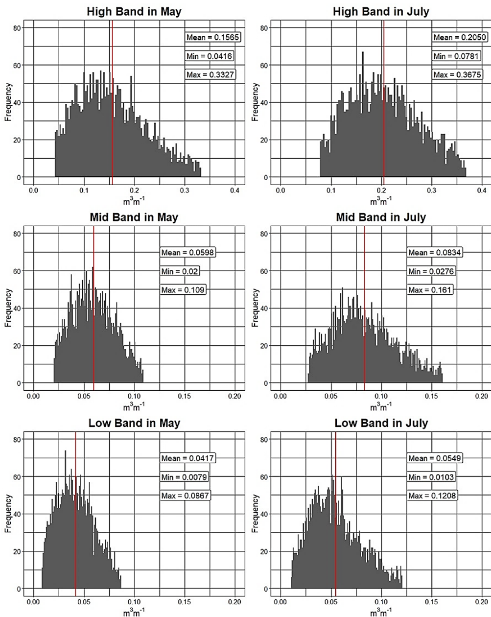
Figure 8. Absolute frequencies of LiDAR measurements of the three bands (Low, Mid, High) with an interval of 0.01 \text{ (m}^3 \text{ m}^{-1}\text{)} . These measurements are part of software output (CSV file) where tractor, coupled with LiDAR, travelled completely four vine-rows. The red line corresponds to the mean value.
