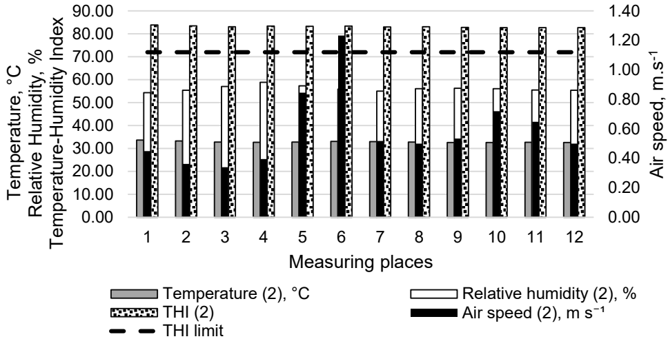
Figure 4. Results of the measured microclimatic quantities in barn 2 with the corresponding temperature-humidity index THI (2).
