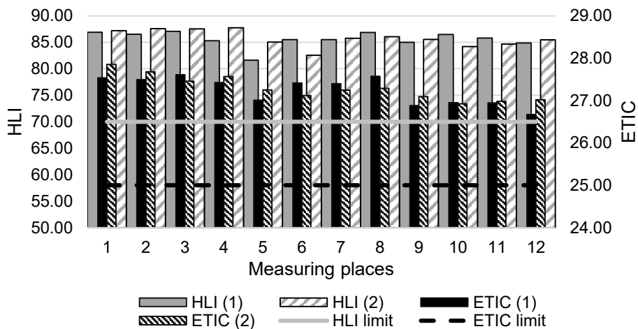
Figure 5. Results of environment evaluation state using HLI and ETIC in both barns.
