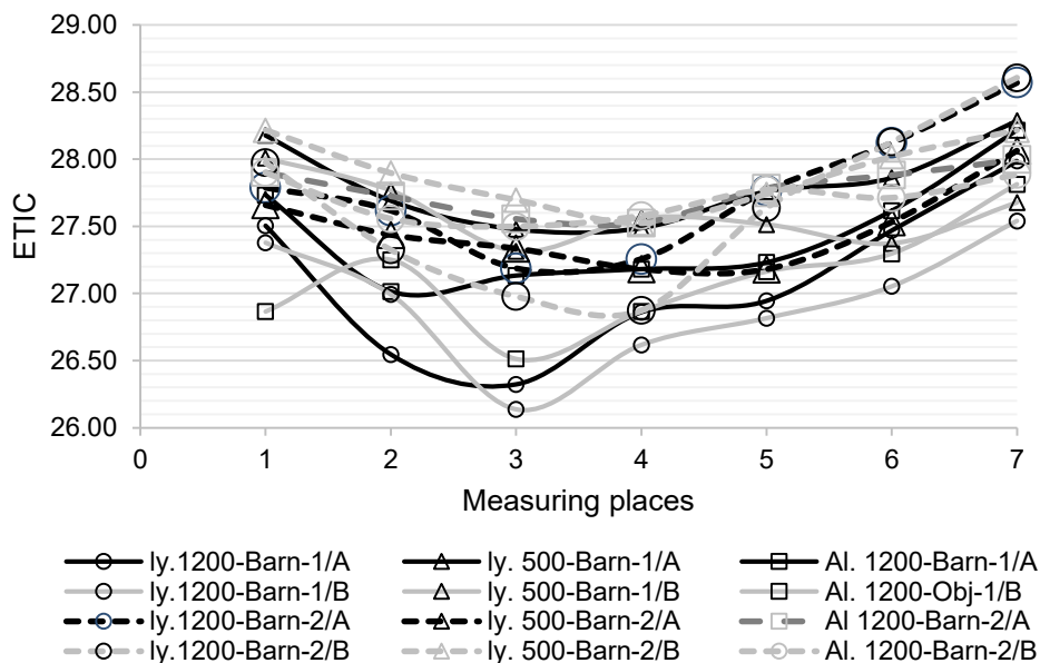
Figure 6. Results of the ETIC evaluation in the longitudinal direction of the barns in the area of adjacent fans (in the lying area at a height of 1,200 mm and 500 mm and in the movement alleys at a height of 1,200 mm – see Fig. 1 and Fig. 2).
