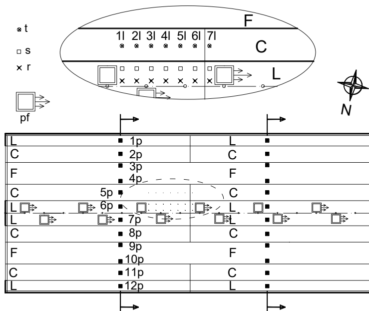
Figure 2. Layout of barn 2 with locations of panel fans and measuring points.
