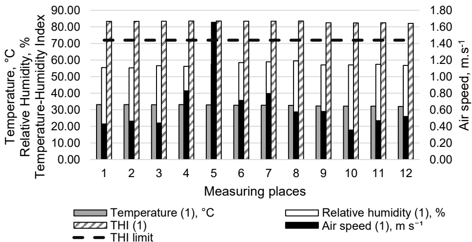
Figure 3. Results of the measured microclimatic variables in barn 1 with the corresponding temperature-humidity index THI (1).
