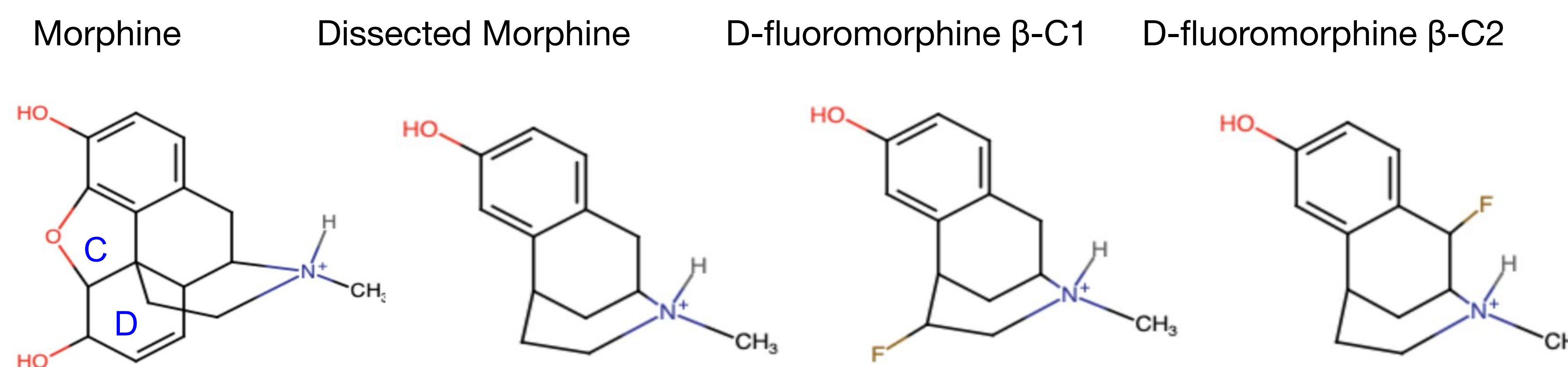
Fig. 2. 2D-line drawings of morphine, dissected morphine, and the \beta -fluorinated morphine derivative candidates, D-fluoromorphine \beta -C1 and D-fluoromorphine \beta -C2.
