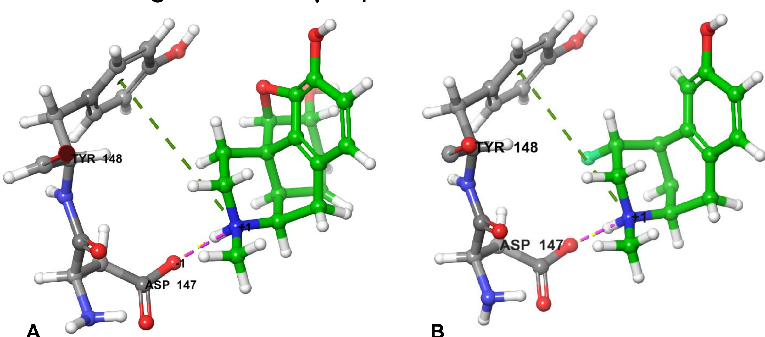
Fig. 1. Fig.1A shows optimized interactions between morphine and Asp147 and Tyr148 within the MOR. Fig.1B shows the interactions between D-fluoromorphine \beta -C1 and Asp147 and Tyr148 within the MOR.
