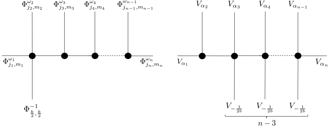
Figure 1: Scheme of the H_3^+ -Liouville correspondence. On the left, an n -point string scattering amplitude in \text{AdS}_3 in which the total winding number is \omega \equiv \omega_1 + \omega_2 + \dots + \omega_n = 1 ; it is defined as an (n + 1) -point correlation function in the SL(2, \mathbb{R})_k WZW model involving one (as \omega = 1 ) spectral flow operator. On the right, the corresponding (2n - 3) -point correlation function in LFT involving n - 2 - \omega degenerate fields V_{-1/(2b)} integrated on the sphere.
