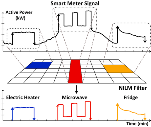
Fig. 5. NILM process.
