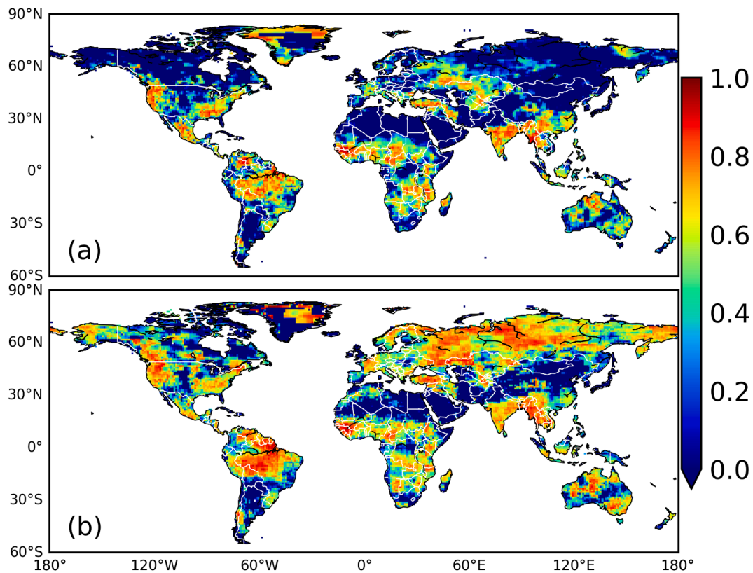
Fig. 7. The maximum NSE values (among three lagged months, t-2 , t-1 , t ) (a) between the standardized GRACE TWSA and CPC soil moisture and (b) between the standardized GRACE and Noah TWAs during the testing periods (April 2014–June 2017 and June 2018–August 2020). The data are standardized to exclude the influence of amplitude and magnitude differences.
