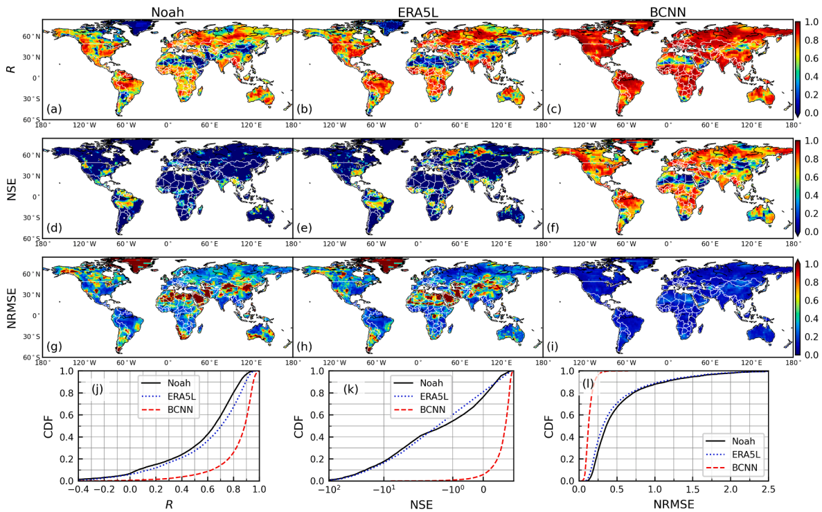
Fig. 4. Spatial maps of R (row 1), NSE (row 2), and NRMSE (row 3) values between the GRACE TWSAs and the Noah- (column 1), ERA5L- (column 2), and BCNN-derived (column 3) TWSAs during the testing periods (April 2014–June 2017, June 2018–August 2020). (j–l) Cumulative distribution functions (CDFs) of the R , NSE, and NRMSE values in (a–i).
