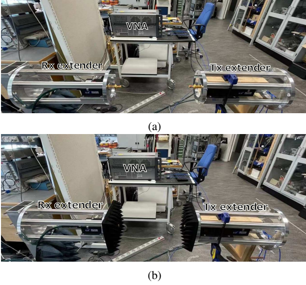
Fig. 7: The photos of the channel measurement setup. (a) The photo of the channel measurement setup without absorber; (b) The photo of the channel measurement setup with absorber.
