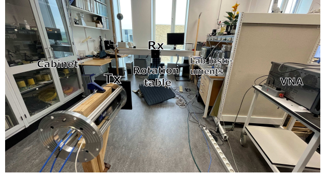
Fig. 9: Picture of the laboratory scenario.
