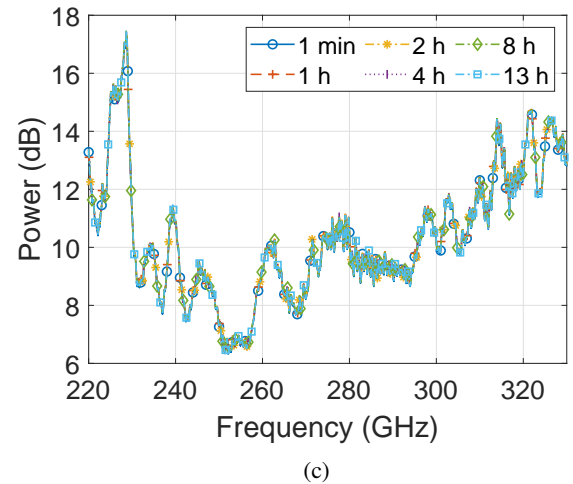
Fig. 6: The results of the stability measurements. (a) The amplitude stability; (b) The phase stability; (c) System response of the channel sounder in the back-to-back measurements over a period of 13 hours.
