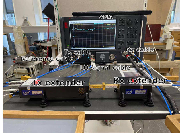
Fig. 4: The photos of the VNA based channel sounder at sub-THz bands. (a) The schematic diagram; (b) The photo of the link budget measurement setup.
