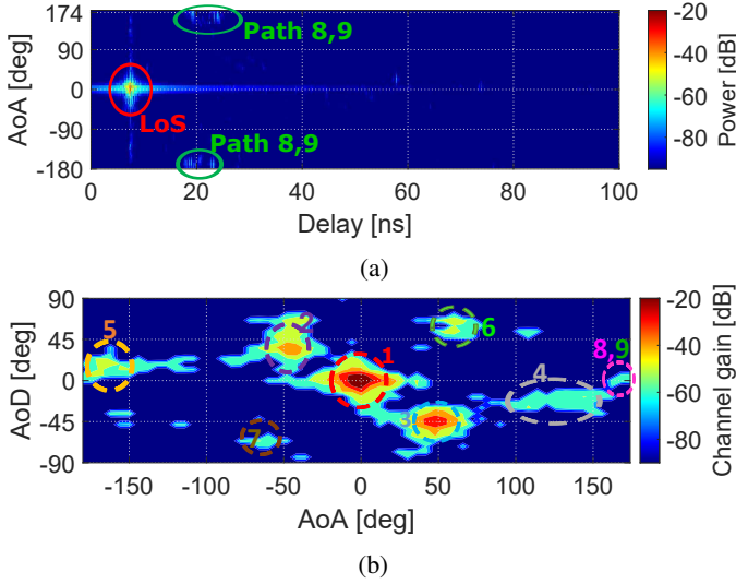
Fig. 10: Double directional measurement results in the lab scenario. (a) The example PDP at the AoD of 0 degree; (b) Power angle spectrum.
