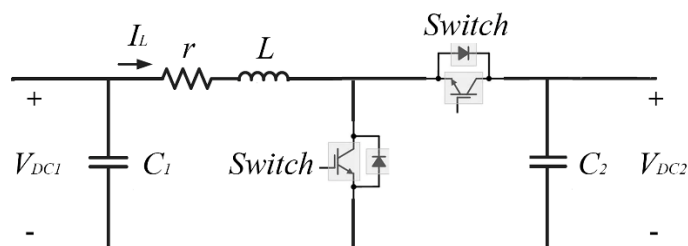
Figure 3. Structure of a bidirectional DC/DC converter.
