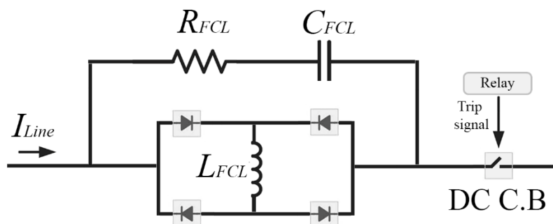
Figure 6. Proposed DC FCL configuration.
