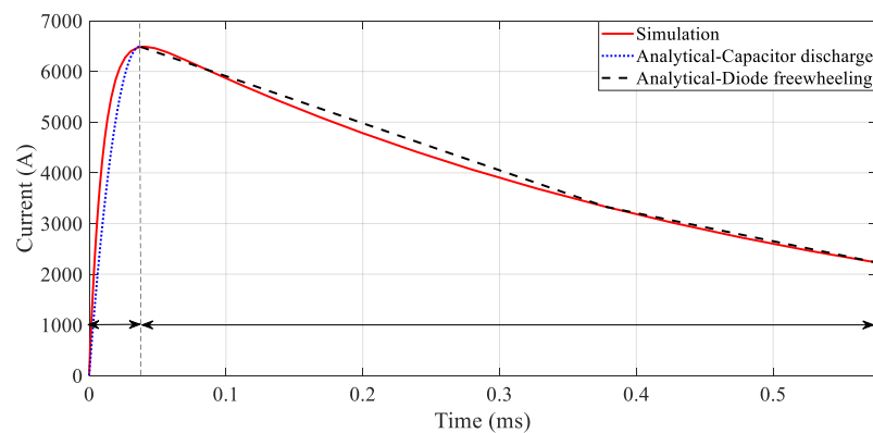
Figure 9. Comparison between analytical and simulation results.
