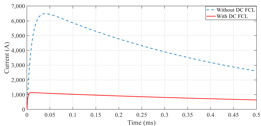
Figure 10. Impact of the DC FCL on the fault current.
