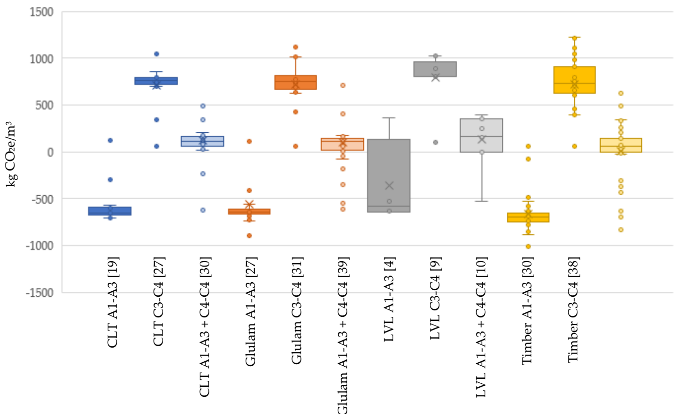
Figure 6. Reported GWP from production (A1–A3), EoL (C3–C4), and total (A1–A3 + C3–C4) from the sample of 81 structural wood product EPDs in accordance with EN 15804. Numbers in brackets indicate the number of data points, i.e., relevant product scenarios included.
