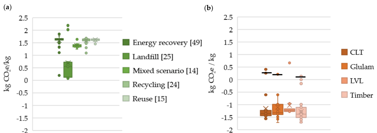
Figure 7. (a) Reported GWP in CO 2 e from different EoL options applied in the surveyed EPDs, normalized to impacts per kg of product. The numbers in brackets indicate the number of data points, i.e., relevant product scenarios included. (b) Reported GWP in CO 2 e from the different categories of structural wood in the surveyed EPDs, normalized to impacts per kg of product. Black marks show GWP further normalized to exclude biogenic CO 2 .
