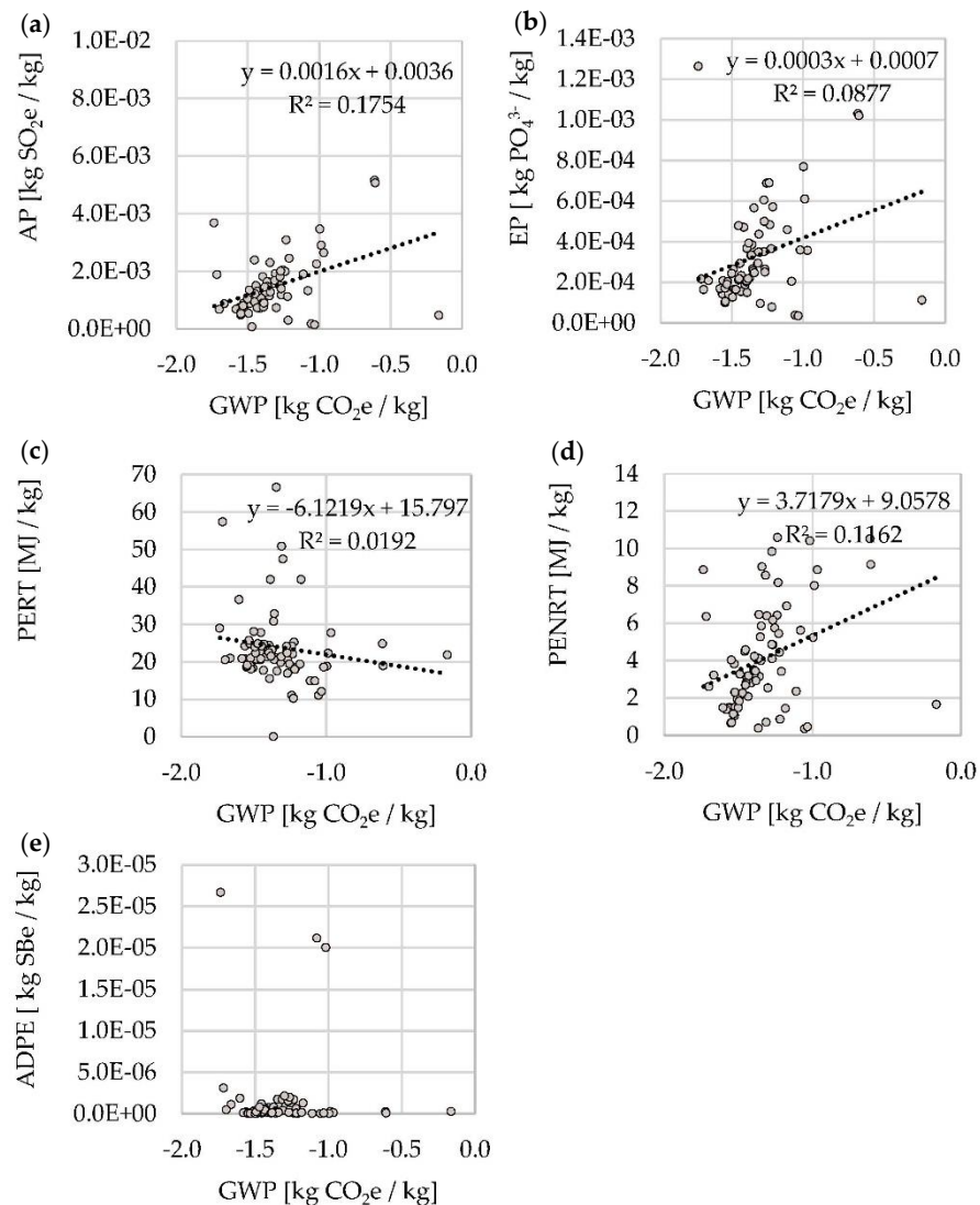
Figure 8. (a) Correlation between GWP and AP for life cycle modules A1–A3. (b) Correlation between GWP and EP for life cycle modules A1–A3. (c) Correlation between GWP and PERT for life cycle modules A1–A3. (d) Correlation between GWP and PENRT for life cycle modules A1–A3. (e) Correlation between GWP and ADPE for life cycle modules A1–A3.
