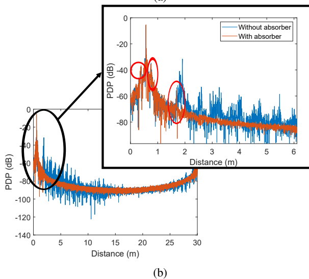
Fig. 4: The comparison of the CIRs with and without absorbers at the distance of 0.4 m. (a) 100 GHz channel sounder; (b) 300 GHz channel sounder.
