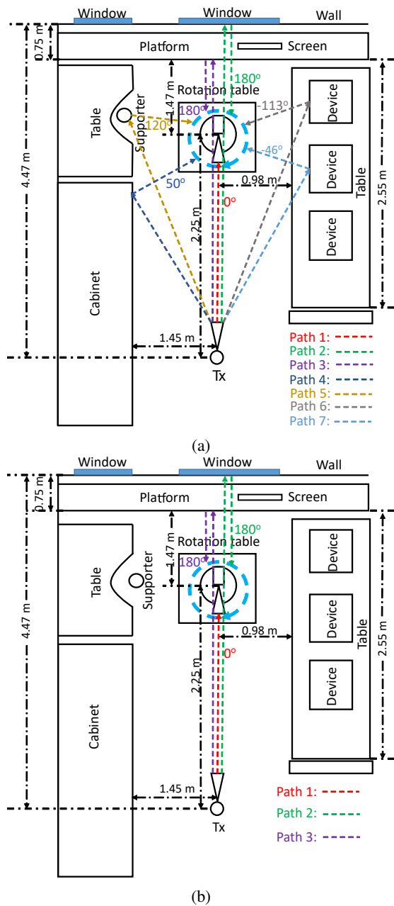
Fig. 7: Relation of the main MPCs to the scenario. (a) 90-110 GHz; (b) 220-330 GHz.
