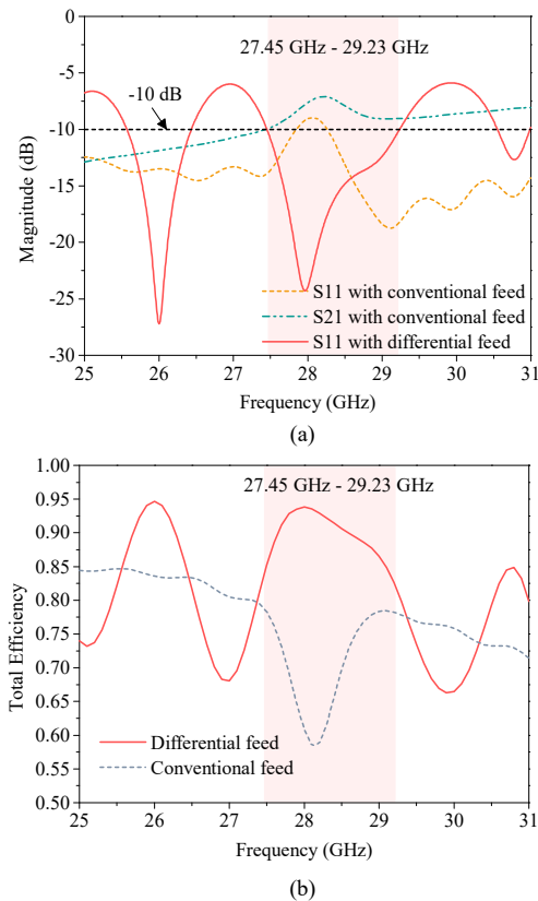
Fig. 9. Simulated performance of 1-D LWA array excited by the conventional and the differential feed. (a) S-parameters. (b) Total efficiencies.
