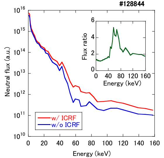
FIG. 5. The energy distributions of neutral flux with and without ICRF heating, measured by CNPA. The green line shows the flux ratio of with and without ICRF heating.
