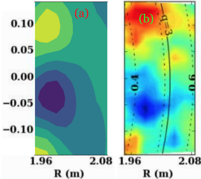
Figure 12. Comparison of n = 4 RSAE mode GTC simulation data and experimental ECEI data for DIII-D #159243 at 807.3 ms. 2D structure on a poloidal plane of \delta T_e/T_{e0} for (a) GTC simulation data, after being processed through the Synthetic-Diagnostic-Platform, and (b) experimental ECEI data.
