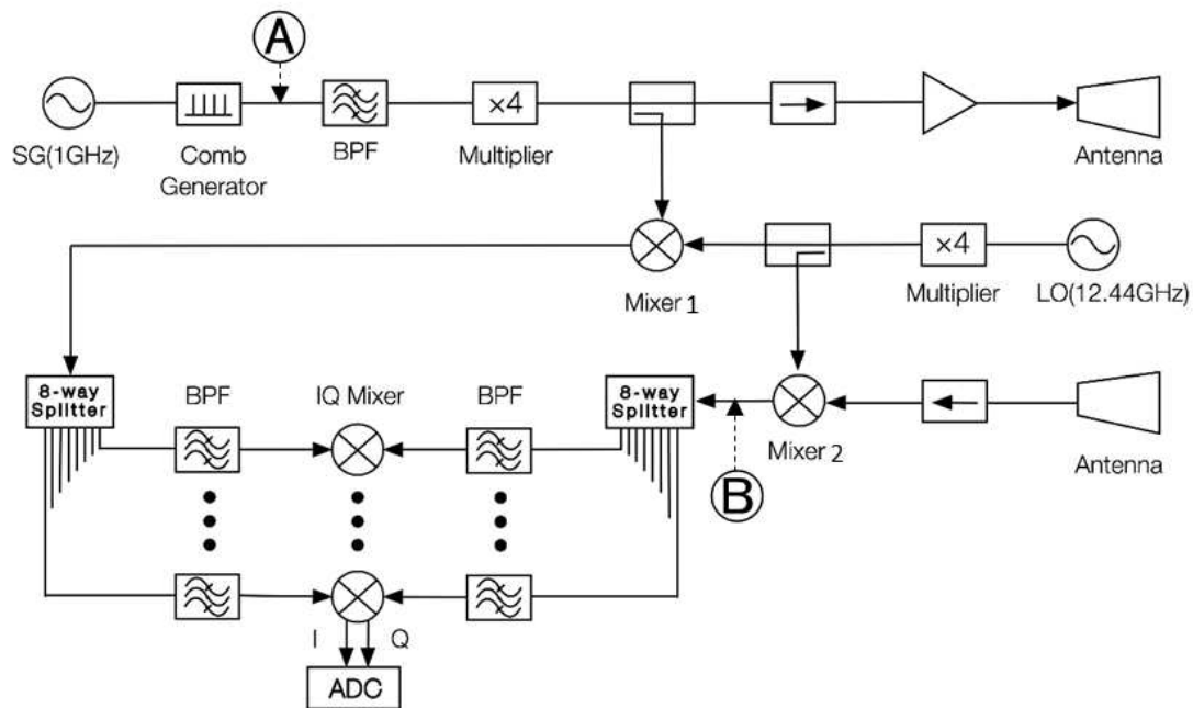
Figure 1. Schematic drawing of U-band microwave reflectometer circuit consisting of a comb generator.
