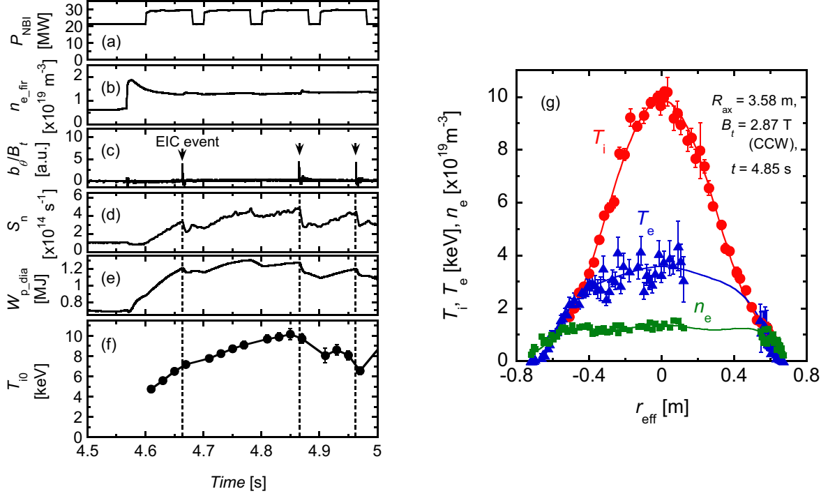
FIG. 5. The time evolution of (a) P_{\text{NBI}} , (b) n_{e_{\text{fir}}} , (c) b/B_t , (d) the neutron emission rate S_n (e) W_{p_{\text{dia}}} , (f) T_{i0} , and (g) the radial profiles of T_i , T_e , and n_e of the highest- T_i plasma in the LHD.
