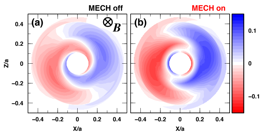
Figure 6. Reconstructed mode structure in the poloidal cross section in (a) MECH turned off phase and (b) MECH turned on phase. Axes X/a and Z/a represent the horizontal distance and the vertical distance from the magnetic axis normalized by the plasma averaged minor radius, respectively.
