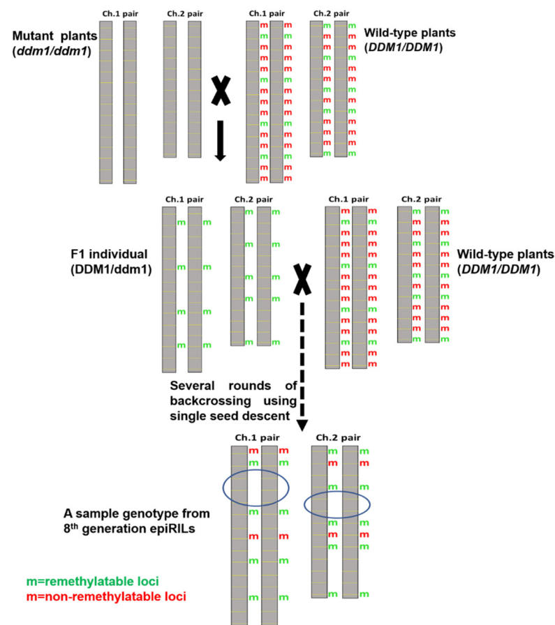
Figure 2. A flowchart illustrating a scheme for the development of epigenetic recombinant inbred lines (epiRILs). Circled loci are examples of loci that do not regain methylation after the introduction of the wild-type DDM1 gene, resulting in the formation of new epialleles.
