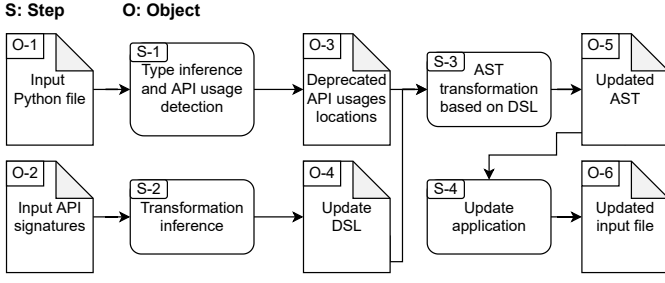
Fig. 1. MLCatchUp Architecture
