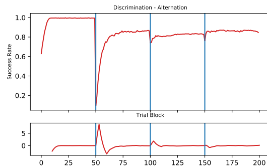
Fig. 7: The agent learns task A (discrimination) for the first 50 episodes, then task B (alternation) for the next 50 episodes, followed by a switch to task A and then back to task B. The presentation of the cues interferes with the learning of the task. A simple method of performance monitoring to identify a rule change can be maintaining a running mean of the rewards obtained over the last n episodes
