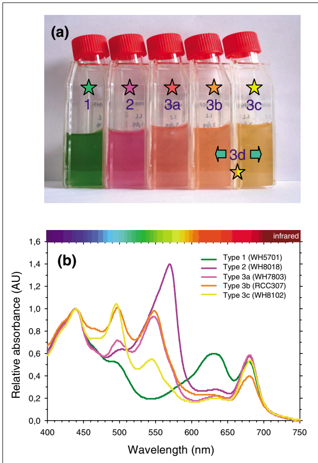
Figure 1 The diversity of pigment types among marine Synechococcus spp. (a) Photograph of representative cultured strains of the major pigment types (1-3) and subtypes (3a-c) of marine Synechococcus grown under low white light and (b) corresponding absorption properties of whole cells. Pigment subtype 3d corresponds to type IV chromatic adapters, which are able to modify their PBS pigmentation from subtype 3b when grown under white or green light to subtype 3c when grown under blue light. The different colors of stars in panel A are a code for the different pigment types.
