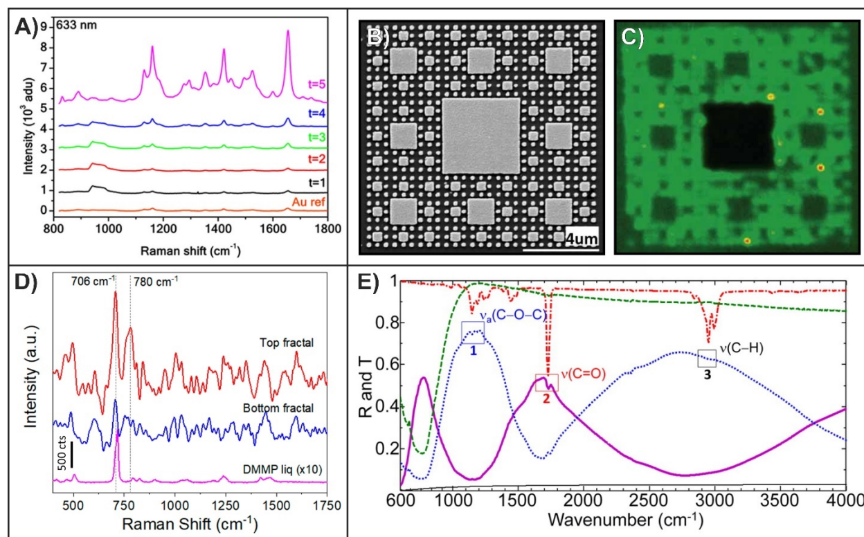
Fig. 8 A) SERS spectra of brilliant cresyl blue coated Sierpiński carpets for first- through fifth-order generations and a reference Au film. 75 B) SEM image of a fourth-order Sierpiński carpet and C) SERS map of a cyanine dye coated surface. 69 D) SERS spectra of a 3-dimensional fractal exposed to dimethyl methylphosphonate (DMMP). 137 A normal Raman spectrum of DMMP in liquid is included for comparison. E) Reflectance (solid purple line) and transmittance (dashed blue line) SEIRA spectra of PMMA coated fifth-order generation Cesaro-type fractal. 95 Reflectance (solid black line) and transmittance (dashed green line) of a 10 nm thick layer of PMMA on CaF 2 and reflectance (red dashed line) spectrum of a gold film coated with a 600 nm thick layer of PMMA are included for reference. Reproduced and adapted with the permission of Ref. 95, 75, 69, and 137. Copyrights 2016 and 2018 American Chemical Society, 2010 Wiley and Sons, and 2018 MDPI respectively.
