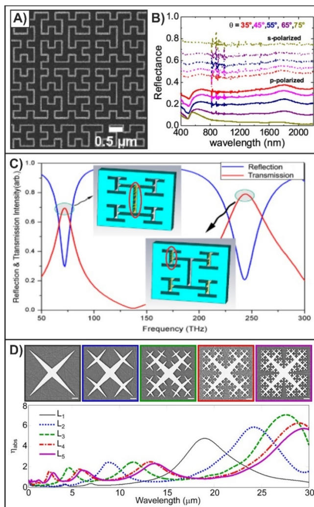
Fig. 4 A) SEM image of part of a ninth-order Hilbert fractal and B) experimental reflectance spectra measured with p- and s-polarized light at varying angles of incidence. 85 C) Transmission and reflectance spectra of a perforated metallic film with an H-Tree fractal. The insets show the electric field distributions at the two resonances. 87 D) SEM images of different generations of Cesaro-type fractals and corresponding calculated absorption cross-section spectra. 95 Reproduced and adapted with permission from Ref. 85, 95. Copyrights 2015 and 2016 American Chemical Society respectively.
