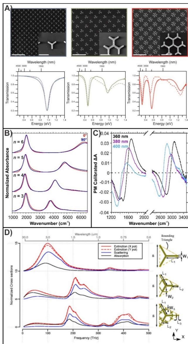
Fig. 2 A) SEM images and transmission measurements for three branched first-, second-, and third-order dendritic fractals. 58 The scale bars in the array images are 2 \mu\text{m} , and 300 nm in the inset images. B) Normalized absorbance spectra for second-order dendritic fractals with varying numbers of inner branches ( n ) using linearly polarized synchrotron light. 59 C) Calibration polarization modulated spectra for three branched second-order dendritic fractals with varying side lengths. 60 D) Spectral variation of the first through third-order generation Ternary tree fractal. 61
