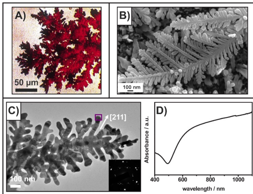
Fig. 1 A) Optical image of dendritic microstructures prepared by pulsed-current deposition of copper. 42 B) SEM image of silver dendrites on a copper substrate prepared by galvanic replacement. 45 C) TEM image gold nanodendrites prepared using a poly(ionic liquid) method. 50 D) absorbance spectrum of the gold nanodendrites. Reprinted and adapted from Ref. 42, 50, and 45. Copyrights Elsevier 1998 and 2017, and The Royal Society of Chemistry respectively.
