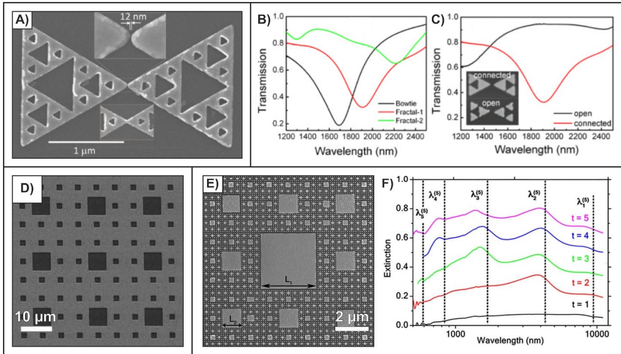
Fig. 3 A) SEM image of a third-order generation Sierpiński triangle. 62 Transmission spectra comparing B) nanoprism bowties, first- and second-order generation Sierpiński triangles and C) Sierpiński triangles with open and connected nanoprisms. 65 D) SEM image of a gold thin film perforated with a Sierpiński carpet pattern. 68 E) SEM image of an inverted Sierpiński carpet with isolated nanostructures and F) extinction spectra of the various fractal generations where t = 1 is just the large central structure and t = 5 is the fractal as shown E. 75 Reproduced and adapted with permission from Ref. 62, 68, and 75. Copyrights 2011 John Wiley and Sons, 2008 AIP Publishing, and 2018 American Chemical Society respectively.
