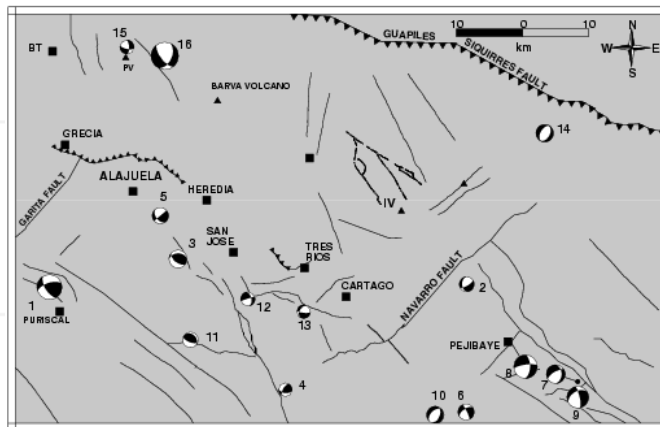
Figure 12. Faulting and focal mechanisms. Small lettered stereo projections are fault-plane solutions for 16 carefully selected earthquakes. BT: Bajos del Toro, PV: Poas Volcano, IV: Irazu Volcano.
