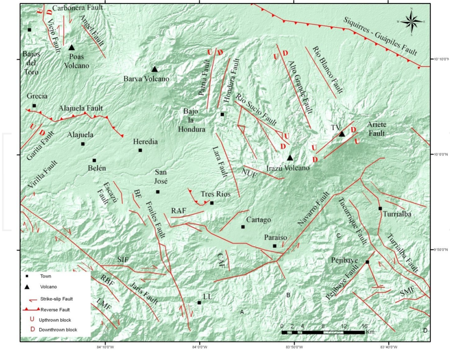
Figure 4. Faults mapped in Central Costa Rica. Triangles mark volcanoes; squares show cities or towns. The aligned volcanoes mark the longitudinal axis of the Central Volcanic Range. The cities of Cartago, San José, Heredia and Alajuela are located in the Central Valley of Costa Rica. The Escazú and Aguacaliente (AF) faults define the southern boundary of the Central Valley. Faults located southeast of the Navarro fault belong to the Talamanca Cordillera. PF: Picagres Fault, BF: Belohorizonte Fault, RAF: Río Azul Fault, SIF: San Ignacio Fault, RBF: Resbalon Fault, LMF: La Mesa Fault, CIF: Cipreses Fault, NUF: Nubes Fault, CAF: Cangreja Fault, SMF: Simari Fault, ATF: Atirro Fault, PCF: Pacuare Fault, LL: La Lucha, SP: Santiago de Puriscal, U/D: normal faults showing relative motion: U, upthrown block; D, downthrown block. Sawteeth along solid lines indicate thrust fault. Strike-slip arrows represent strike-slip faults.
