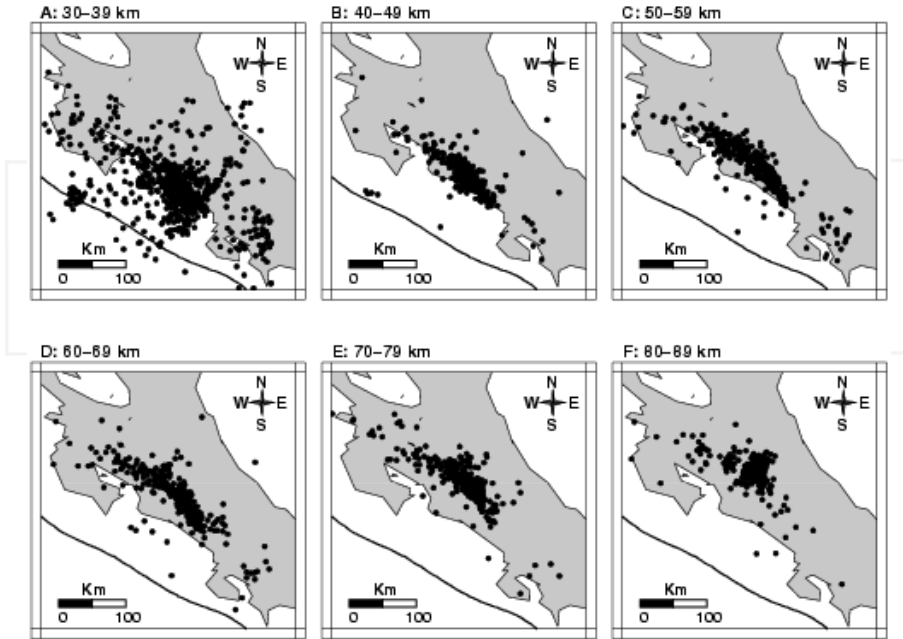
Figure 10. Cumulative numbers of located earthquakes, separated into six depth ranges, within or near the Costa Rican territory. These graphs plot earthquakes detected and located by the Red Sismologica Nacional (RSN: ICE-UCR) from 1992 to 2009. Depth ranges are in km.
