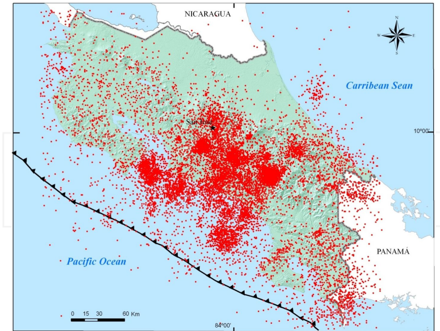
Figure 9. Background seismicity in Costa Rica from 1992 through 2009. Circles are earthquakes. Several clusters represent the most important seismic zones of Costa Rica. The sum of these clusters generates a zone of concentrated seismicity in Central Costa Rica. MAT: Middle American Trench.
