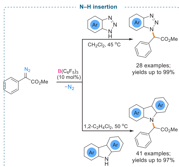
Scheme 11. B(C_6F_5)_3 Catalyzed N–H Insertion of Benzotriazole (Top) and Carbazole (Bottom) Using \alpha -Aryl \alpha -Diaoesters
