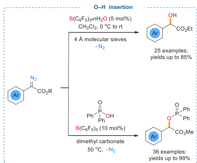
Scheme 9. B(C_6F_5)_3 Catalyzed O–H Insertion into \alpha -Aryl \alpha -Diazoesters (Top) and O–H Insertion of \alpha -Aryl \alpha -Diazoesters into Phosphinic Acids (Bottom)
