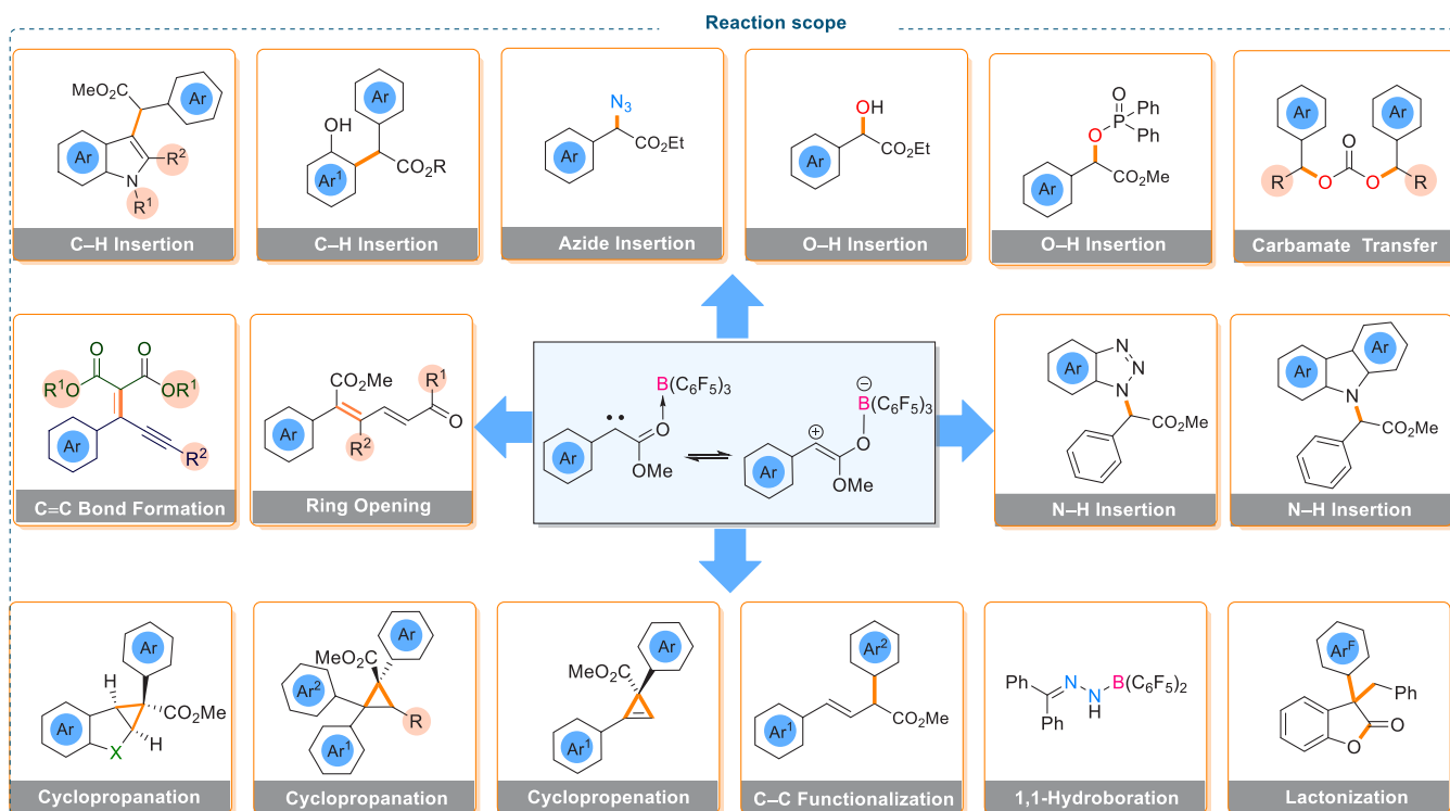
Scheme 8. Generic Overview of B(C_6F_5)_3 Activation of Diazo Compounds and Subsequent Reactivity
