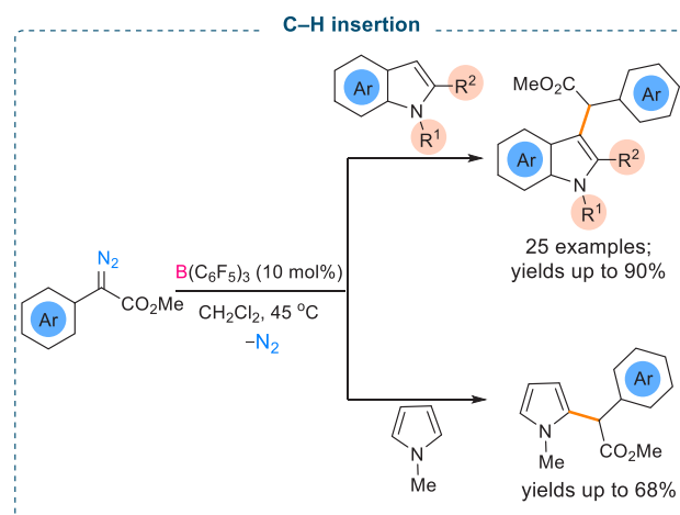
Scheme 12. B(C_6F_5)_3 Catalyzed C–H Insertion of Indoles and Pyrroles with \alpha -Aryl \alpha -Diaoesters
