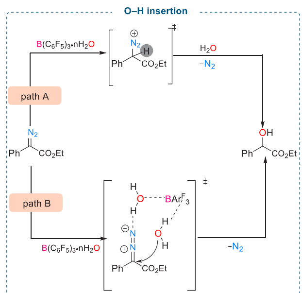
Scheme 10. Mechanistic Details of B(C_6F_5)_3 Catalyzed O–H Insertion into \alpha -Aryl \alpha -Diazoesters
