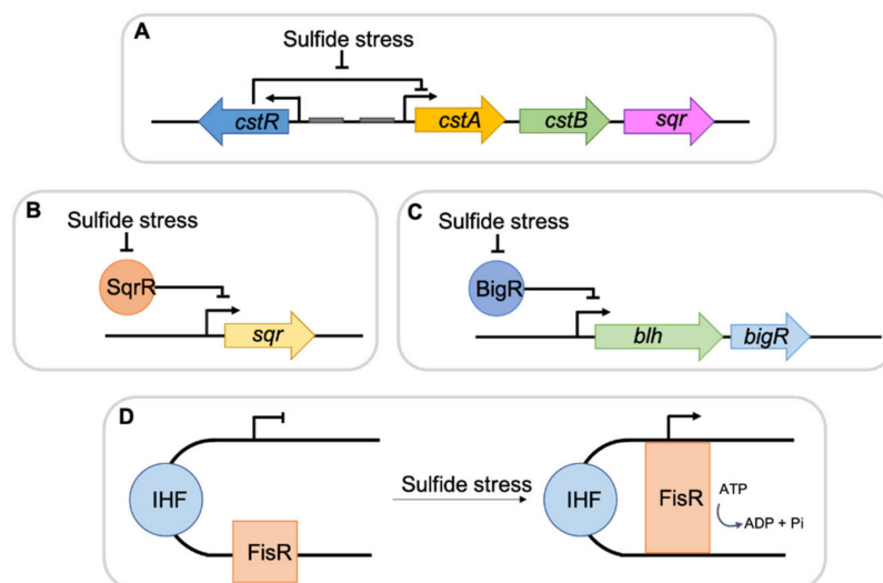
Figure 1. General scheme summarizing bacterial H 2 S regulators. (A) CstR regulator binds to the upstream region of the cst genes repressing their expression. During sulfide stress, the DNA-binding affinity of the repressor decreases allowing for RNA polymerase binding and gene transcription. (B,C) SqrR and BigR bind to promoter regions of sqr , blh and bigR genes, inhibiting transcription. In the presence of sulfide, the repression is lifted and genes expression occurs. (D) Under sulfide stress, FisR hydrolyzes ATP to ADP plus free phosphate, resulting in RNA polymerase activation and increase in gene expression.
