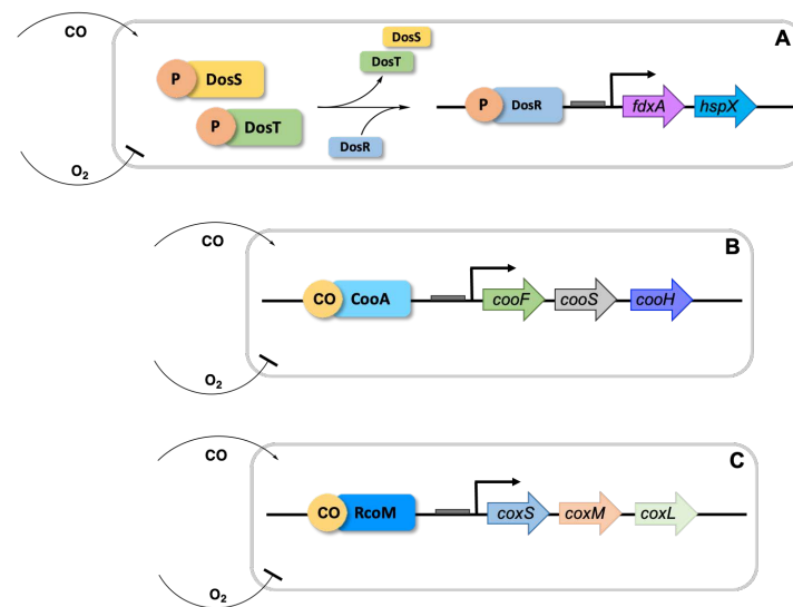
Figure 2. General scheme on the action of CO regulators. (A) Upregulation of the dormancy of DosR-phosphate transcriptional regulator is triggered by CO and H 2 S. (B,C) The CooA and RcoM regulators, which are activated by CO, upregulate the transcription of the coo and cox gene products that catalyze conversion of CO to CO 2 .
