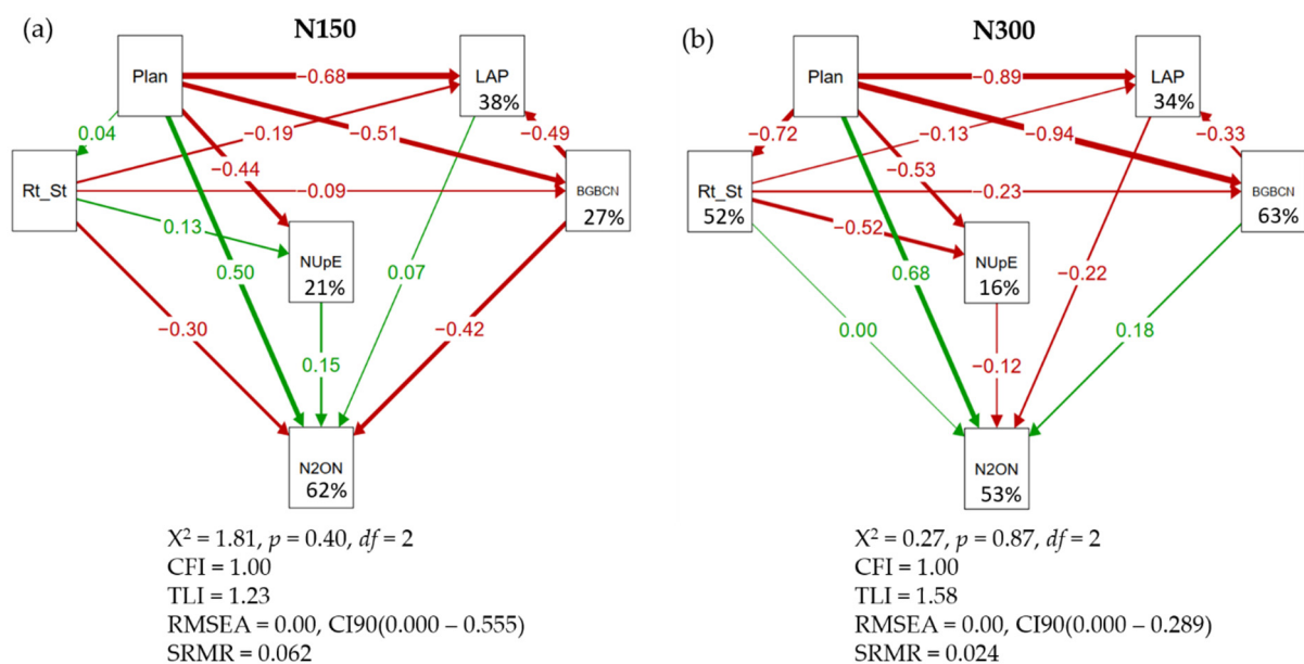
Figure 5. Structural equation models showing the relationships between the measured variables at (A) the N150 fertilizer rate and (B) at the N300 fertilizer rate. Plan—forage plantain proportion; NUpE—whole plant N uptake; Rt_St—root/shoot ratio; BGBCN—belowground biomass C/N ratio; LAP—leucine aminopeptidase, a proxy for microbial activity; green arrows represent a positive association, and red arrows represent a negative association; numbers within arrows represent standardized path coefficients, whereby negative path coefficients indicate a negative relationship. The higher the absolute value of the path coefficient, the more important is the path. Numbers in the white boxes show the percentage of explained variance of each of the endogenous variables. X^2 indicates the fit of the model, Comparative Fit Index (CFI), Tucker Lewis Index (TLI), and the Root Mean Square Error of Approximation (RMSEA).
