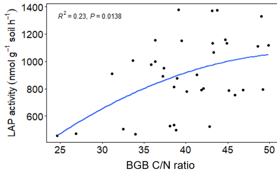
Figure 3. A quadratic response curve showing the relationship between the microbial enzyme (LAP) activity and belowground biomass C/N ratio.
