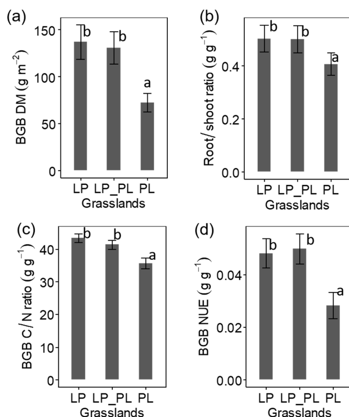
Figure A2. Sward effect on (a) the belowground (BGB) DM yield, (b) root/shoot ratio, (c) BGB C/N ratio and (d) BGB nitrogen use efficiency (NUE). Differing letters indicate significant differences ( p < 0.05 ); error bars indicate standard errors of the mean.
