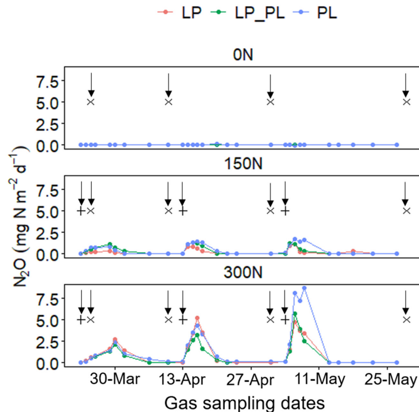
Figure 4. Graphs showing daily N_2O fluxes from the diverse swards at different fertilization rates. LP represents Lolium perenne ; PL represents Plantago lanceolate . Arrows with + represent fertilizer application events, and arrows with x represent a biomass harvesting event.
