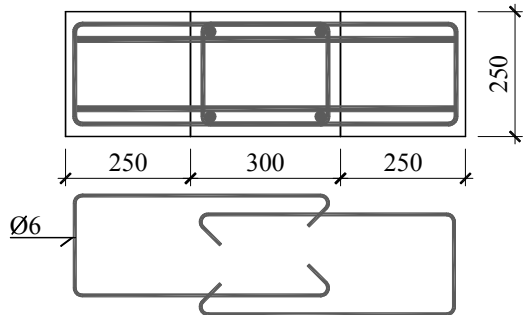
Zbrojenie modelu / Specimen's reinforcement
