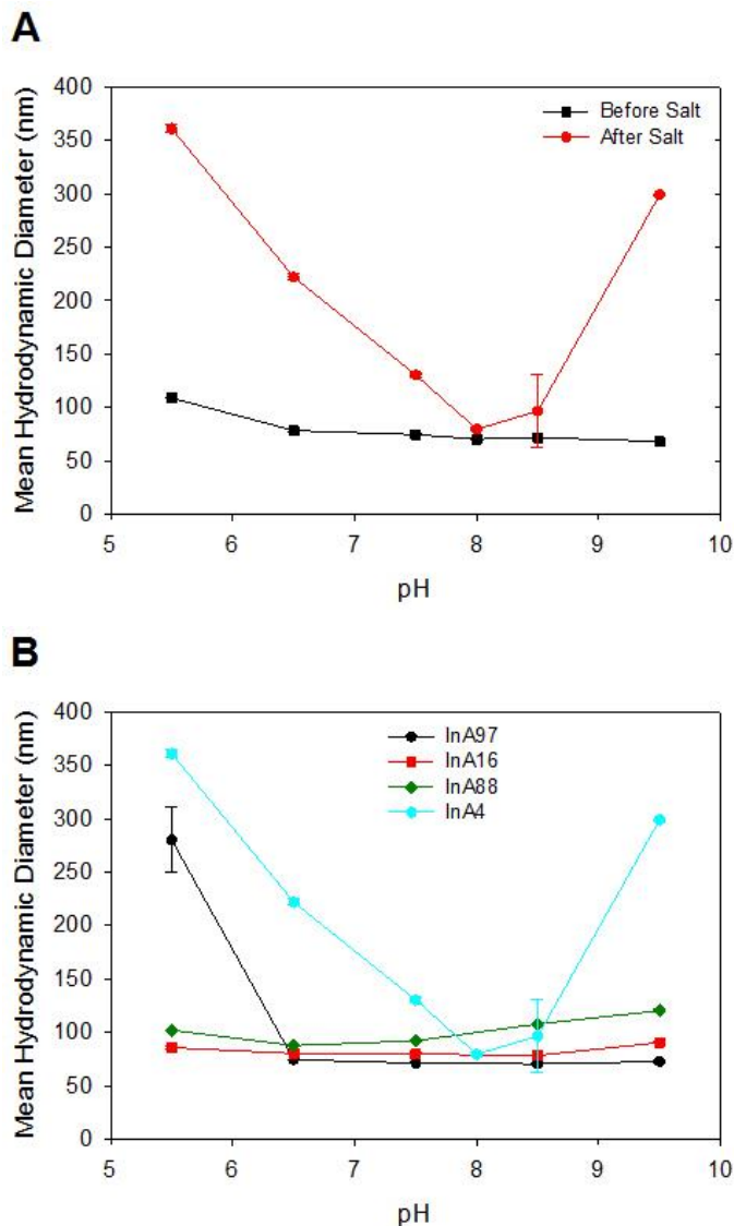
Figure 11. DLS aggregation curves to assess pH-dependent adsorption of mAb onto AuNP. The mAb concentration is fixed at 30 \mu\text{g}/\text{mL} . (A) Mean hydrodynamic diameter of InA4-AuNP conjugate as a function of pH before and after addition of 1% NaCl. (B) Mean hydrodynamic diameter of four mAb-AuNP conjugate as a function of pH after addition of 1% NaCl. Each data point is the average of 3 independent experiments with standard deviations presented by error bars.
