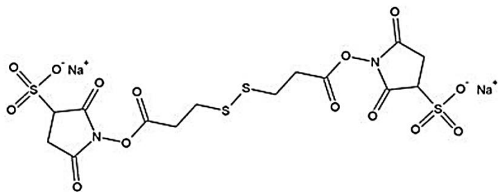
3,3'-dithiobis(sulfosuccinimidyl propionate)
