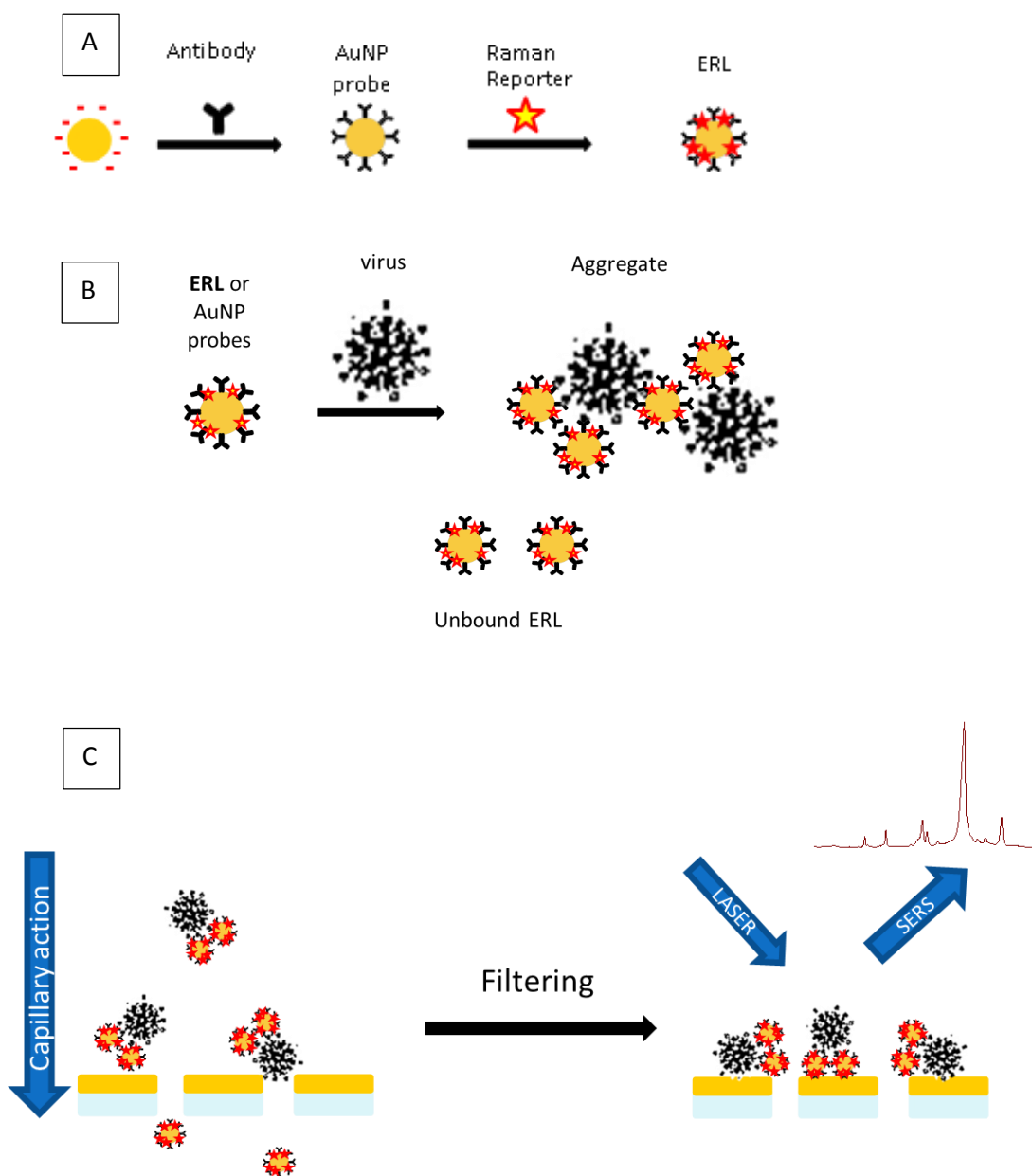
Figure 9. Schematic illustration of one-step homogeneous immunoassay coupled with SERS analysis. (A) Immobilization of Raman reporter and antibody molecules to synthesize AuNP probes or ERLs, (B) Virus-induced aggregation of ERLs in solution, (C) Filtration to separate aggregates from unbound ERLs to concentrate SERS signals.
