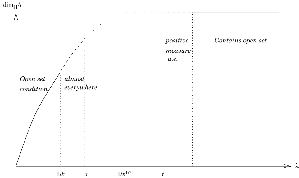
FIGURE 1. Extending the regions where dimension is known.
