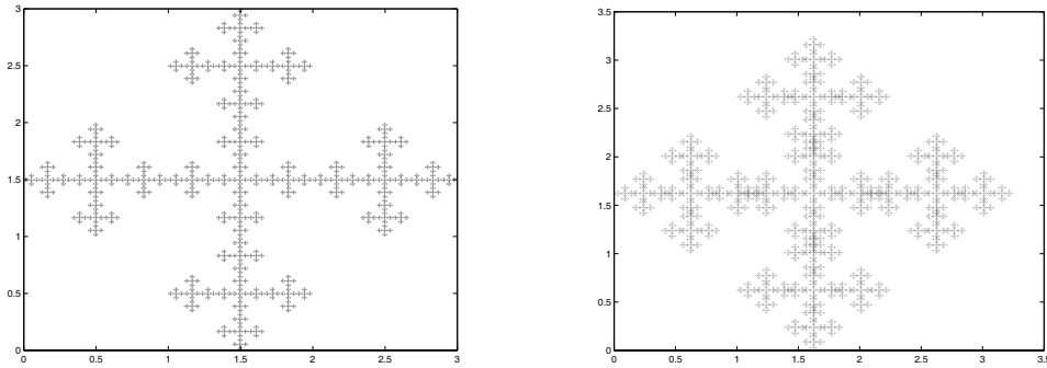
FIGURE 4. Vicsek sets where (i) \lambda = 1/3 and (ii) \lambda = 0.386 .
