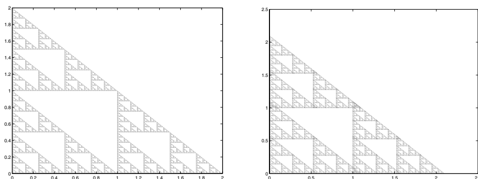
FIGURE 2. Sierpinski gasket where (i) \lambda = 0.5 and (ii) \lambda = 0.525 .
