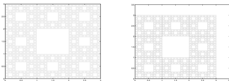
FIGURE 3. Sierpinski carpets where (i) \lambda = 1/3 and (ii) \lambda = 0.338 .
